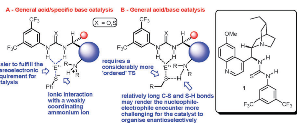
Fig. 1 Organocatalytic Michael-type additions involving thiols.
