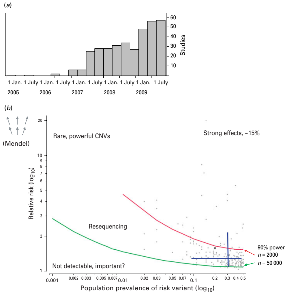
Fig. 2. Properties of genome-wide association study (GWAS) findings from the literature. (a) Quarterly temporal trends in the publication of GWAS. (b) The accumulated GWAS literature on human diseases. The x axis is the population prevalence of a risk variant and the y axis the relative risk conferred (both using a log 10 scale to provide separation). The gray points show the prevalence–risk combination for all single nucleotide polymorphism (SNP) associations for human complex diseases with p < 5 \times 10^{-8} . Power curves are shown for 1000 cases/1000 controls (red line) and 25 000 cases/25 000 controls (green line). The blue lines depict the 10th–90th percentiles from the GWAS literature for allele frequency (horizontal line) and relative risk (vertical line). The intersection of the blue lines is the median population prevalence (0.3) and relative risk (1.25).
