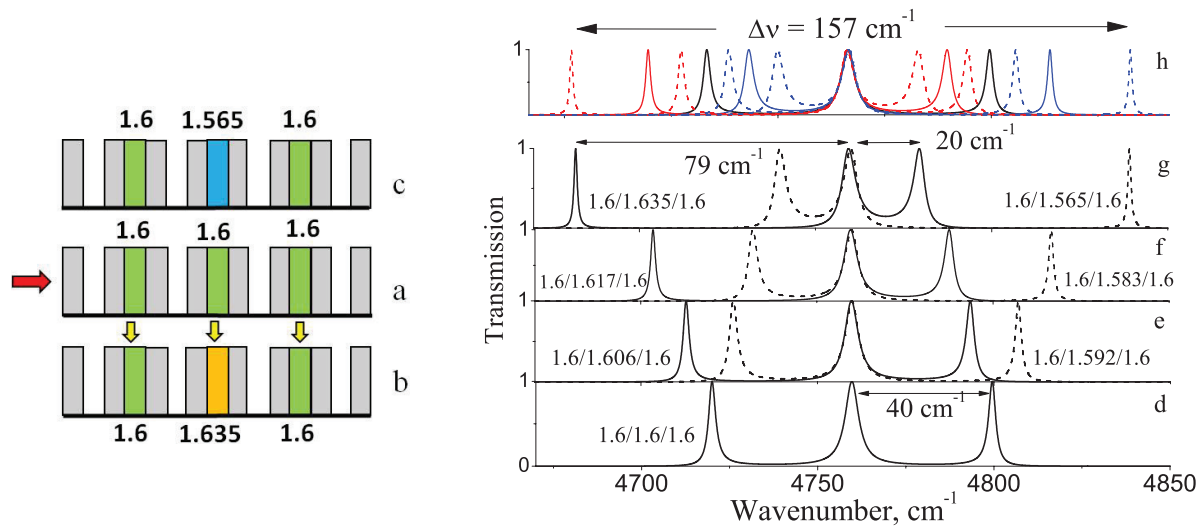
FIGURE 5 | (a–c) Tuning of the n_c filler in the central cavity only; (d–g) 7 triplets in the 3rd SB, realized with different n_{C2} (shown by numbers at the peaks) with a fixed central peak and tuned lateral (edge) resonances, (h) summing peaks for all states of n_c .
