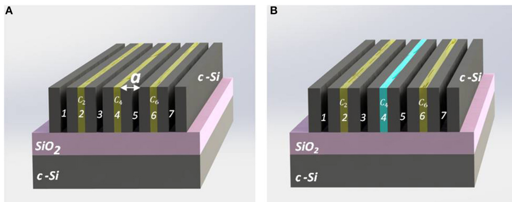
FIGURE 1 | (A) Schematic diagram of 1D PhC based on a Si-air structure with three central air channels (c2, c4, and c6) infiltrated with a nematic liquid crystal (LC) of tunable refractive index, n_c . (B) Schematic diagram of 1D PhC in which the refractive index of the central cavity n_{c4} is changed without changing n_c in the edge cavities, giving a new sequence of n_c . The notation a stands for the lattice constant of the 1D PhC and is equal to a sum of the thicknesses of crystalline Si (c-Si) rib, d_{Si} , and the air (or LC) channel, d_{air} .
