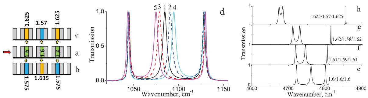
FIGURE 6 | (a–c) Schematic diagram illustrating cross-tuning of the n_c filler, (d) 5 triplets in the 1st SB with fixed edge peaks and a tunable central peak, (e–h) the original triplet and 3 triplets in the 3rd SB, demonstrating the split into a doublet and a mono-peak. Numbers at the peaks are the values of n_c for the fillers in the cavities of the resonators. In panel (d) the numbers beside the curves correspond to the following set of n_c : 1 – 1.6/1.6/1.6; 2 – 1.585/1.62/1.585; 3 – 1.615/1.58/1.615; 4 – 1.575/1.63/1.575; 5 – 1.625/1.57/1.625.
