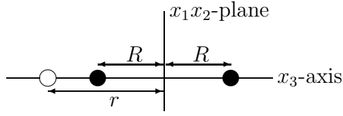
Figure 3: The monopole configuration for the point dyon metric calculation, the solid dots represent (1, -) -monopoles, the other dot is the (-, 1) -monopole.
