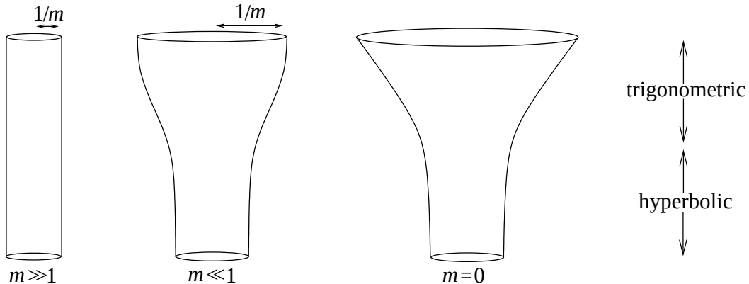
Figure 2: The axially symmetric moduli space for differing values of m
