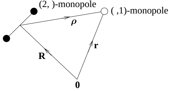
Figure 1: An illustration of the definition of the various separation vectors.
