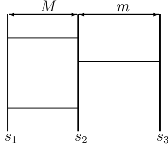
Figure 4: (2, 1) Hanany-Witten configuration with vertical fivebranes and horizontal threebranes.
