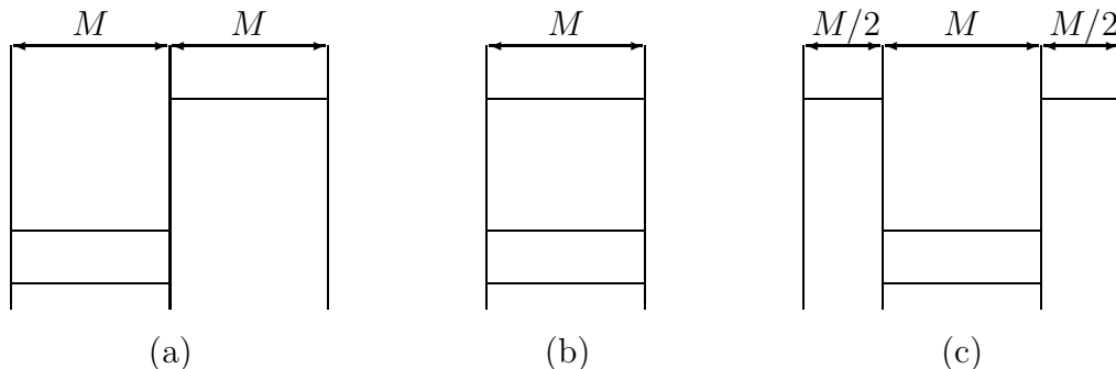
Figure 5: Hanany-Witten configurations illustrating the discussion of two monopoles close together and one far away. (a) corresponds to a (2,1) -monopole where m = M . (b) corresponds to a 3-monopole, the topmost threebrane is far away from the other two. (c) corresponds to a (1,2,1) -monopole.
