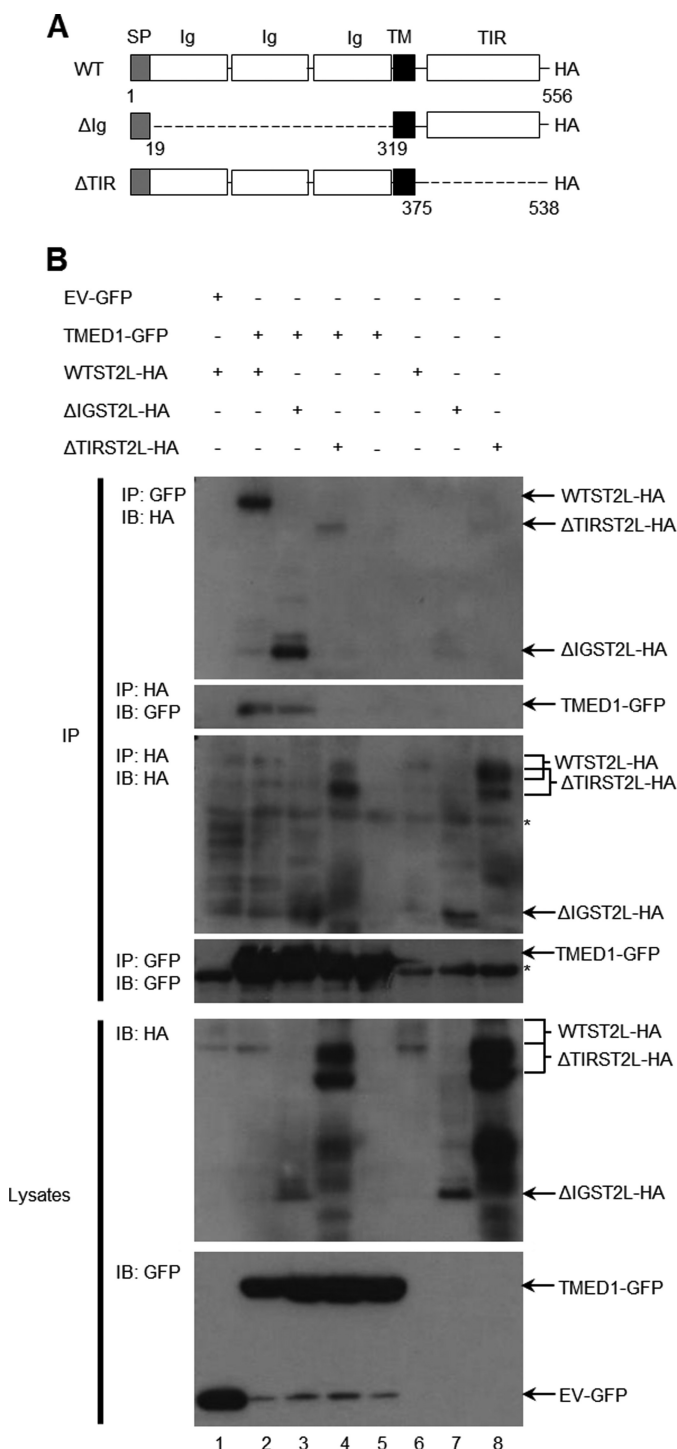
FIGURE 2. The TIR domain of ST2L is required for the TMED1/ST2L interaction. A, schematic representation of full-length and truncated ST2L-HA constructs tested for their ability to bind TMED1-GFP. SP, signal peptide; Ig, immunoglobulin domain; TM, transmembrane domain. B, HEK-293T cells were transfected with plasmids encoding empty vector-GFP or TMED1-GFP along with wild-type ST2L-HA or truncated ST2L constructs (ΔIGST2L or ΔTIRST2L). 48 h following transfection, cells were lysed, 50 μl was kept as the whole cell lysate, and the remainder was immunoprecipitated (IP) with anti-GFP or anti-HA antibody-coupled Protein A/G Plus-agarose beads for 3 h at 4 °C. Whole cell lysates and immunoprecipitated samples were analyzed by Western blotting using anti-GFP and anti-ST2L antibodies. Asterisks indicate antibody heavy chain bands. Results presented are representative of three independent experiments. IB, immunoblot.
