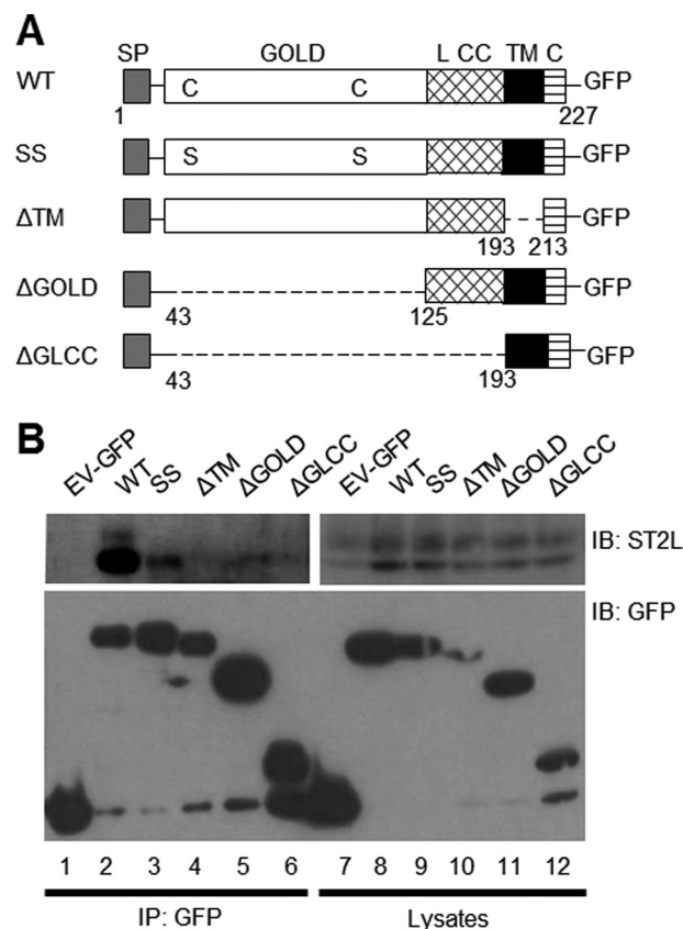
FIGURE 3. The GOLD domain of TMED1 is required for the TMED1/ST2L interaction. A, schematic representation of full-length, mutated, and truncated TMED1-GFP constructs tested for their ability to bind ST2L. SP, signal peptide; L CC, linker and coiled-coiled domain; TM, transmembrane domain; C, C-terminal tail. B, HEK-293T cells were transfected with plasmids encoding empty vector-GFP (EV-GFP), wild-type TMED1-GFP (WT), TMED1-GFP mutant (SS), or truncated constructs (ΔTM, ΔGOLD, or ΔGLCC) as shown. 48 h post-transfection, cells were lysed, 50 μl was kept as the whole cell lysate, and the remainder was immunoprecipitated (IP) with GFP-Trap beads for 1–2 h at 4 °C. Whole cell lysates and immunoprecipitated samples were analyzed by Western blotting using anti-GFP and anti-ST2L antibodies. Results presented are representative of three independent experiments. IB, immunoblot.
