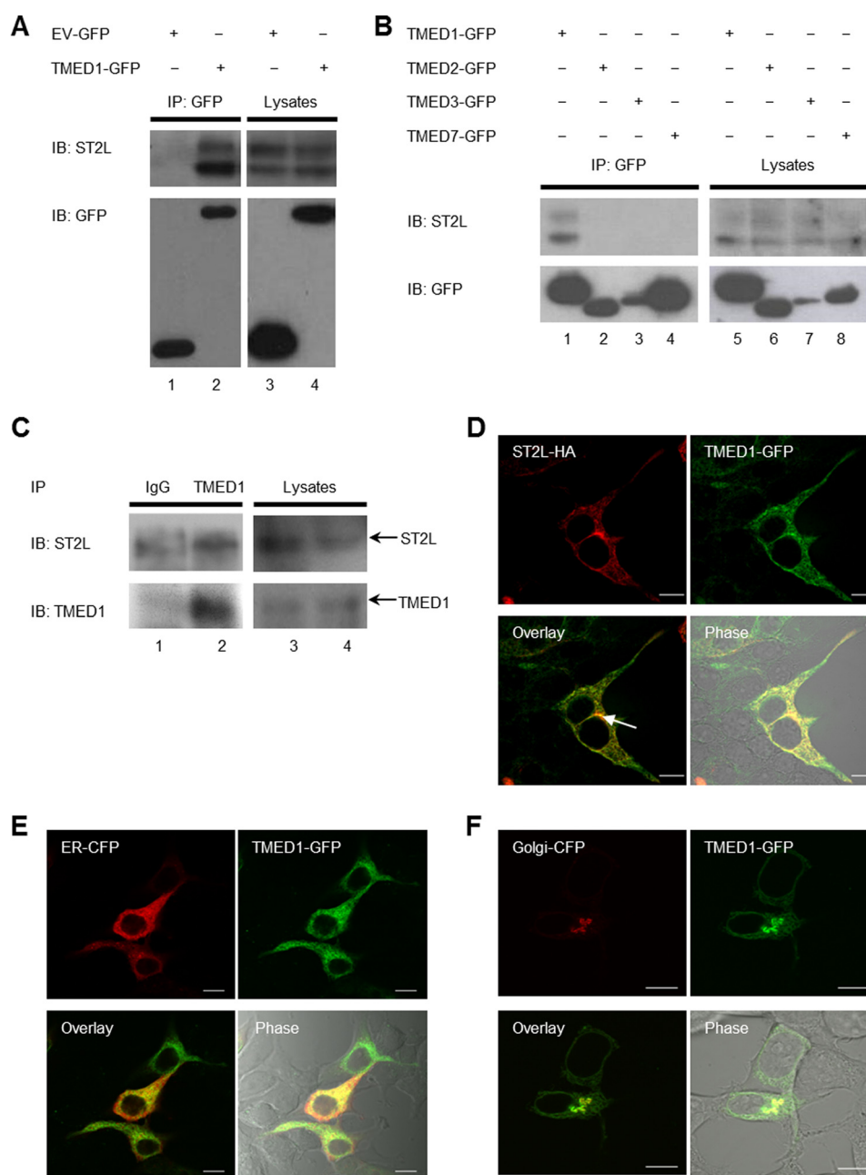
FIGURE 1. TMED1 and ST2L interaction. A and B, HEK-293-hST2L cells were transfected with plasmids encoding empty vector-GFP, TMED1-GFP, TMED2-GFP, TMED3-GFP, or TMED7-GFP as indicated. 48 h post-transfection, cells were lysed, 50 \mu l was kept as the whole cell lysate, and the remainder was immunoprecipitated (IP) with GFP-Trap beads for 1–2 h at 4 °C. Whole cell lysates and immunoprecipitated samples were analyzed by Western blotting using anti-GFP and anti-ST2L antibodies. Results presented are representative of five (A) and two (B) independent experiments. IB, immunoblot. C, 2 \times 10^7 HMC-1.1 cells were lysed, and 50 \mu l was kept as the whole cell lysate. The remainder was immunoprecipitated with anti-rabbit IgG, anti-TMED1, or anti-ST2L antibody-coupled Protein A/G Plus-agarose beads for 2 h at 4 °C. Whole cell lysates and immunoprecipitated samples were analyzed by Western blotting using anti-TMED1 and anti-ST2L antibodies. Results presented are representative of four independent experiments. D, HEK-293T cells were transiently transfected with plasmids encoding TMED1-GFP and ST2L-HA. 48 h later, cells were fixed, stained with anti-HA antibodies, and visualized by confocal microscopy. Data shown are representative of a total of 70 cells analyzed in three independent experiments. The GFP tag is represented in green, and ST2L-HA is represented in red. HEK-293T cells were transiently transfected with plasmids encoding TMED1-GFP and ER-CFP (E) or TMED1-GFP and Golgi-CFP (F). 48 h later, cells were fixed and visualized by confocal microscopy. Data shown are representative of 82 (E) and 10 (F) cells from three experiments in which a total of 82 cells were analyzed. The GFP tag is represented in green, and the CFP tag is represented in red.
