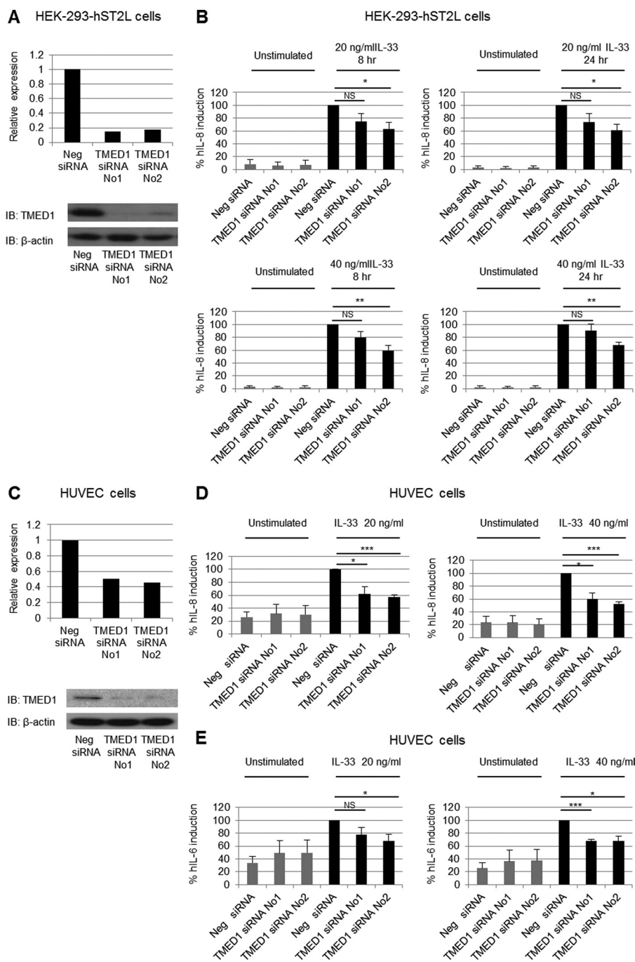
FIGURE 5. TMED1 is involved in IL-33 signaling. HEK-293-hST2L cells (A and B) or HUVECs (C–E) were transfected with control siRNA, TMED1 siRNA-1, or TMED1 siRNA-2. RNA or protein from HEK-293-hST2L cells (A) or HUVECs (C) transfected with siRNA was analyzed by real-time PCR and Western blotting to determine the levels of TMED1 knockdown. mRNA expression was normalized to GAPDH and is presented relative to negative siRNA-transfected cells, which was set to 1. Data in A and C are representative of three independent experiments. IB , immunoblot. 48 h following transfection, HEK-293-hST2L cells (B) or HUVECs (D and E) were stimulated with 20 or 40 ng/ml IL-33 for the times indicated, and supernatants were analyzed by ELISA. Results are expressed as percent human (h) IL-8 or IL-6 induction and represent the mean \pm S.E. of results for three independent experiments, each carried out in triplicate. The asterisks indicate statistical significance (unpaired two-tailed Student's t test): *, p < 0.05 ; **, p < 0.01 ; ***, p < 0.001 . NS, not significant.
