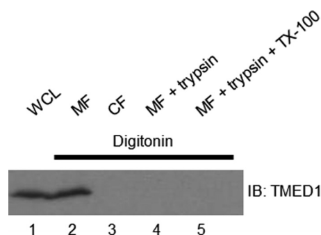
FIGURE 4. The GOLD domain of TMED1 projects into the cytosol. Shown are the results from a biochemical protease protection assay of HEK-293T cells. Lane 1, whole cell lysate (WCL); lane 2, membrane fraction (MF); lane 3, cytosolic fraction (CF); lane 4, membrane fraction plus trypsin; lane 5, membrane fraction plus trypsin plus Triton X-100 (TX-100). Samples were analyzed by Western blotting and probed with anti-TMED1 antibody. Results are representative of three independent experiments. IB, immunoblot.
