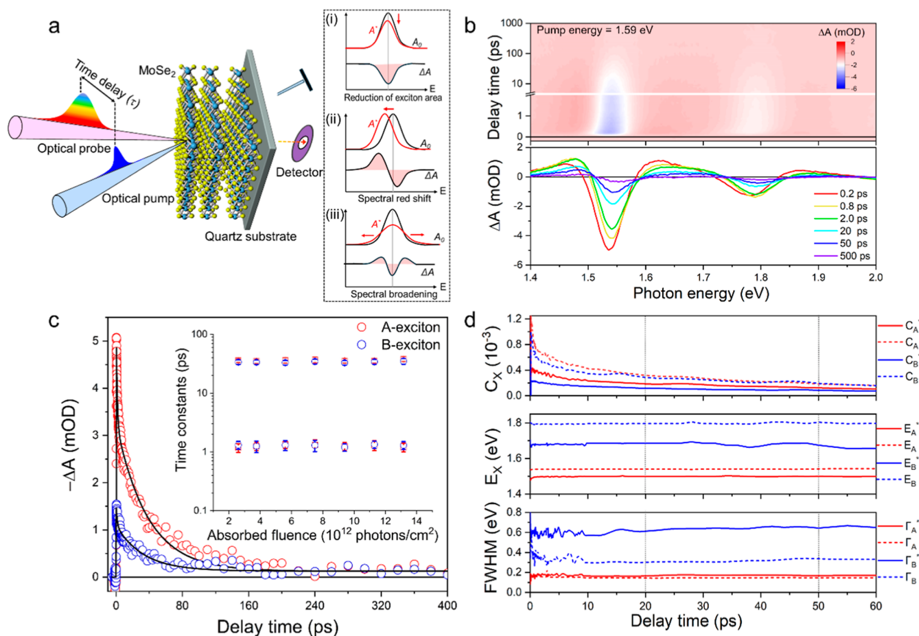
Figure 2. TA spectroscopy at 1.59 eV pump photon energy and absorbed photon fluence of 13.1 \times 10^{12} photons/cm 2 . (a) Schematic of TA experiments. Inset: (i–iii) typical transient effects after photoexcitation (b) TA colormap (upper panel) and corresponding TA spectra at the indicated times (lower panel) (c) Decay kinetics of the bleach probed at 1.54 and 1.78 eV below the A (red circles) and B (blue circles) exciton transitions, respectively. The black solid lines represent a biexponential fit and a constant background with decay times shown in the inset also for other pump fluences. (d) Parameters from fits of superpositions of Lorentzian functions (see text) to TA spectra, showing the evolution of amplitudes ( C_x , upper panel), energies ( E_x , middle panel), and FWHM ( \Gamma_x , bottom panel) for A (red circles) and B (blue circles) transitions.
