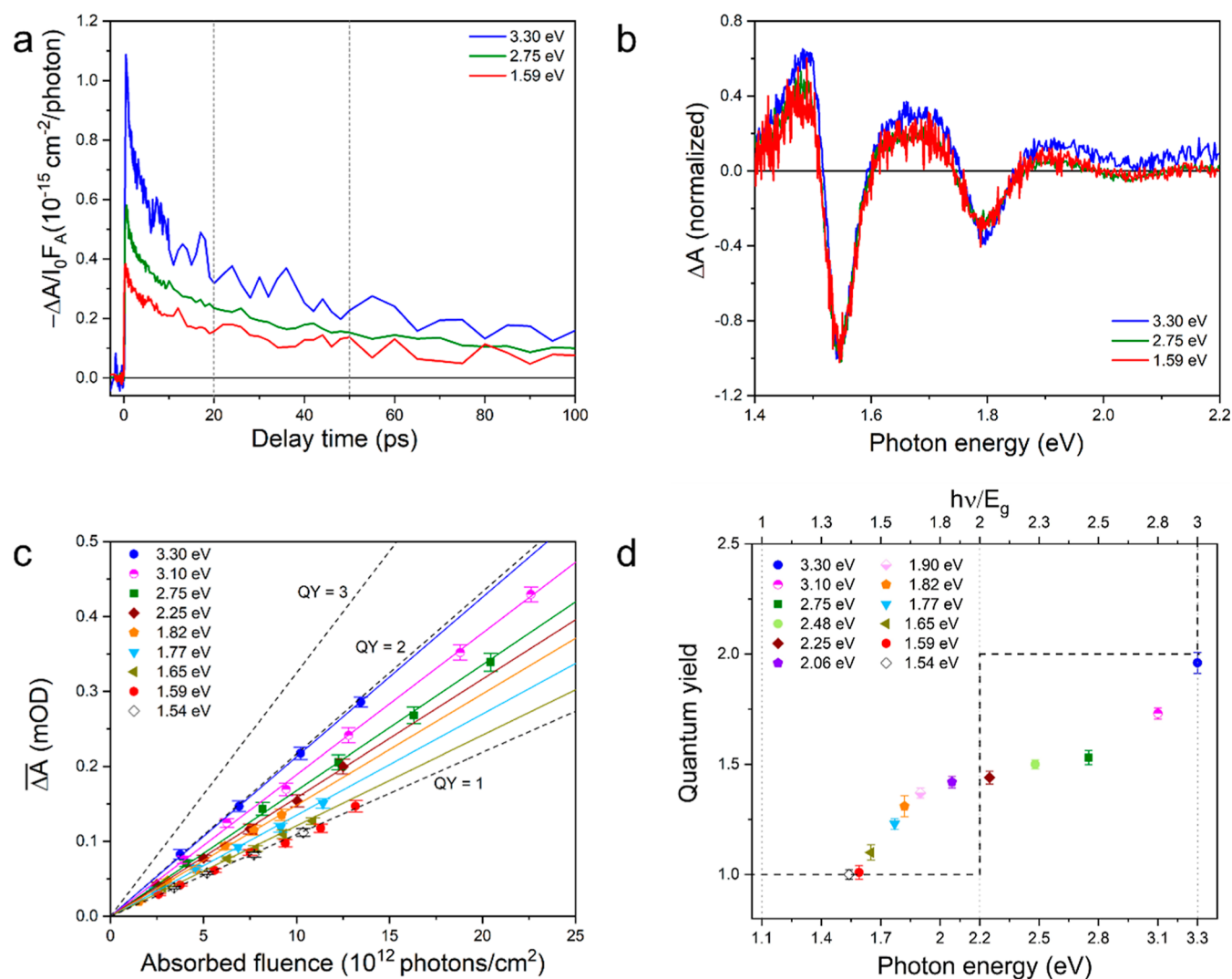
Figure 3. Investigation of CM by TA spectroscopy. (a) Effect of pump photon energy on the decay kinetics of the TA signal normalized to absorbed pump fluence [in the range (3.7\text{--}4.1) \times 10^{12} photons/cm 2 ], recorded at 1.54 eV where the bleach is highest. The vertical gray dotted lines indicate the 20–50 ps time interval used to determine the CM quantum yield. (b) TA spectra normalized at 1.54 eV and averaged over delay times in the range 20–50 ps for different pump photon energies. (c) Integrated absolute TA signal, \Delta A , as a function of absorbed photon fluence for different pump photon energies. The solid lines are linear fits to the experimental data, with their slope representing the quantum yield. Error bars represent the standard deviations. (d) Quantum yields plotted as a function of photon energy (bottom axis) and band gap multiple (top axis). The dashed step-like black curve illustrates the scenario of ideal CM.
