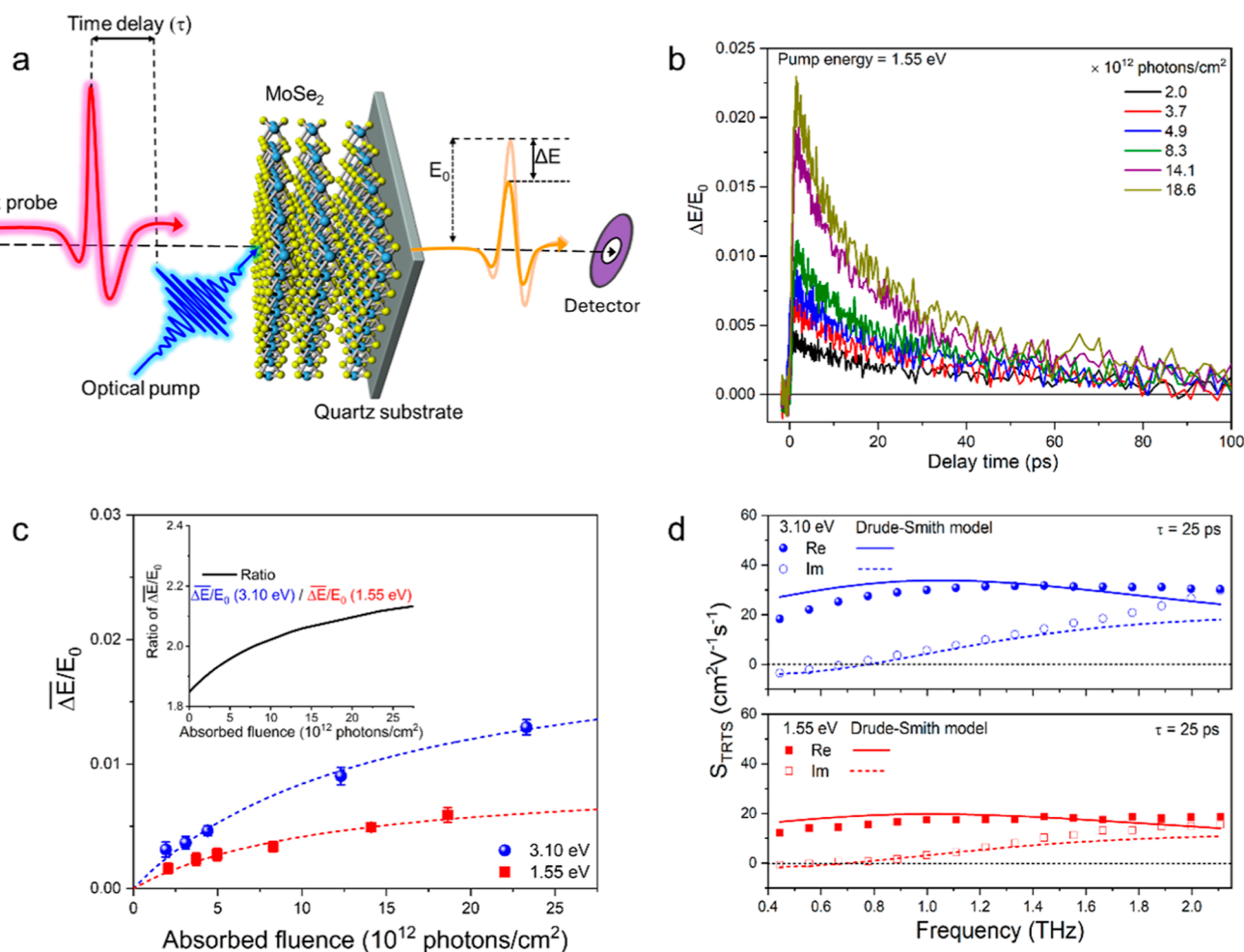
Figure 4. Investigation of CM by THz spectroscopy. (a) Schematic depiction of optical pump-THz probe experiments. (b) Pump fluence-dependent OPTP signals, \Delta E(\tau)/E_0 , upon excitation at 1.55 eV. (c) OPTP signals averaged in the interval 20–50 ps as a function of absorbed photon fluence, following photoexcitation at 1.55 eV (red squares) or 3.10 eV (blue circles). The dotted lines represent fits of the saturation function \Delta E/E_0 = \alpha I/(I + I_s) , and the inset shows the ratio of the fits for 3.10 and 1.55 eV. (d) Frequency-dependent complex photoconductivity signals obtained from TRTS measurements at a delay time \tau = 25 ps after photoexcitation at 1.55 or 3.10 eV and low absorbed photon density of (2.0 \pm 0.1) \times 10^{12} photons/cm 2 . The solid and dotted lines represent fits of the Drude-Smith model to the real and imaginary conductivity components, respectively.
