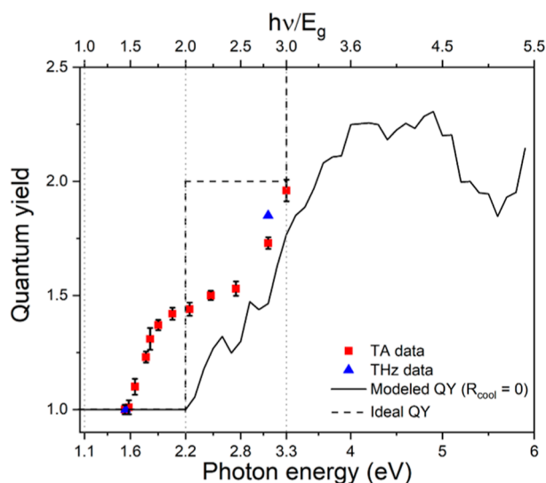
Figure 5. Calculated quantum yield (black solid line) in the absence of carrier cooling, along with experimental data from TA spectroscopy (red squares) and THz conductivity measurements (blue triangles), as a function of photon energy (bottom axis) and band gap multiple (top axis). The black dashed line represents the case of ideal stair-like CM.
