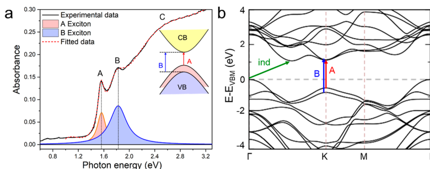
Figure 1. Characterization of the 2H-MoSe 2 thin film. (a) Ground-state optical absorption spectrum (solid black curve). The dashed red curve represents the fit of eq 1 to the absorption spectrum. Inset: Schematic showing the A and B transitions between the two upper valence band (VB) and the lowest conduction band (CB) states. (b) Electronic band structure obtained from DFT calculations, showing transitions at the direct band gap giving rise to the A exciton (red arrow) and B exciton (blue arrow), as well as the transition at the indirect band gap (green arrow).
