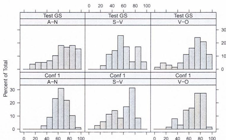
Figure 8.4.1: The distribution of the gold standard numeric score vs. the distribution of the system's first configuration numeric scores.
