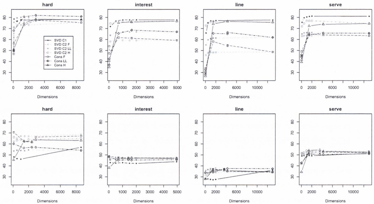
Figure 7.3.1: SVD and consolidation summary – The top of the graph shows supervised experiment results for ambiguous words (hard, interest, line and serve) whilst the bottom of the graph shows unsupervised experiment results for the same set of ambiguous words. The Y axis in all plots represents Accuracy whilst the X axis represents number of dimensions kept. The legend inside the supervised-hard plot applies to all plots.
