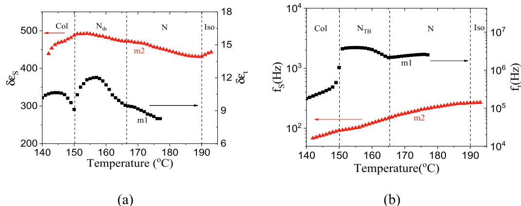
Fig. 12. (a) Plots of the dielectric relaxation strengths, \delta\epsilon_t and \delta\epsilon_s , and the (b) relaxation frequencies f_t and f_s as functions of temperature for the high ( m_1 ) and low frequency modes ( m_2 ).
