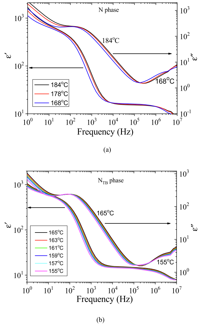
Fig. 11. Permittivity \epsilon' and dielectric loss \epsilon'' of a planar-aligned cell plotted as a function of frequency in (a) N and (b) N_{TB} phases.
