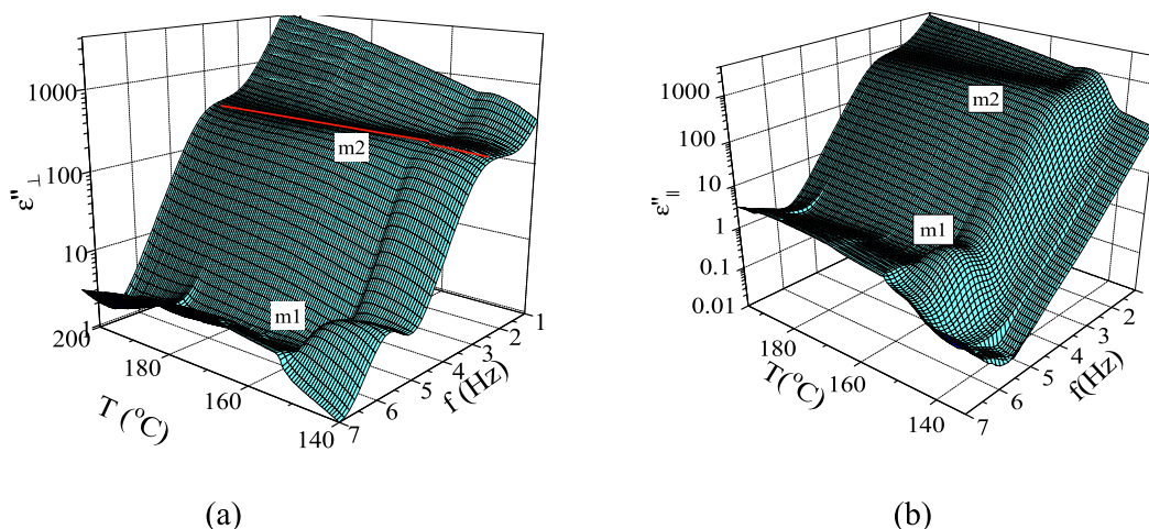
Fig. 8. The three-dimensional (3D) plot of temperature dependent dielectric loss spectra ( \epsilon'' ) for (a) 4 \mu\text{m} planar aligned cell and (b) homeotropic gold plated cells in the frequency range 1 Hz – 10 MHz. The temperature is stabilized to within 0.05^\circ\text{C} .
