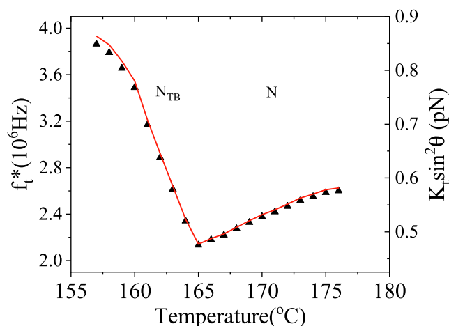
Fig. 13. Temperature dependence of the relaxation frequency of the tilt fluctuation mode ( f_t ). The red line is the line of fitting to eqn. (6). K_t \sin^2 \theta values are deduced from the fit close to the transition temperature.
