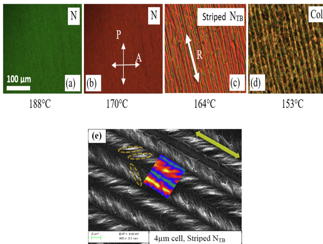
Fig. 3. The POM textures of mesophases in a 15 \mu\text{m} planar aligned cell. The phases indicated are: (a) N at 188 °C, (b) N at 170 °C, (c) N_{TB} at 164 °C (2 °C below the N- N_{TB} transition temperature) and of (d) the Columnar phase at 153 °C and (e) Imaging of the polymerized template of N_{TB} phase in a mixture of CBC7CB and 5 CB (designed for reducing N- N_{TB} transition temperature) in a planar-aligned cell (cell-spacing 4 \mu\text{m} ) using Scanning Electron Microscope (SEM). The left and the right handed molecular packing with twist and bend of the molecules in neighbouring layers is revealed by SEM imaging. The yellow twisted helices seen in Fig. 3(e) correspond to the rope-like structure observed in Fig. 3(c). The procedure of obtaining SEM images is detailed by Panov et al. [21]. Figure 3(e) is reproduced with permission from the authors. The rope like structure obtained by Focal Conic Polarizing Microscopy (FCPM) [19] on a LC sample cell under similar conditions is overlapped on to the SEM polymer template imaging of the N_{TB} structure. The length of the bar shown (in green colour) in Figure 3e is 2 \mu\text{m} .
