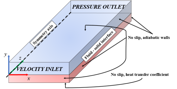
Fig. 4. 3D computational domain and boundary conditions. Blue and red regions are fluid and solid domains respectively.
