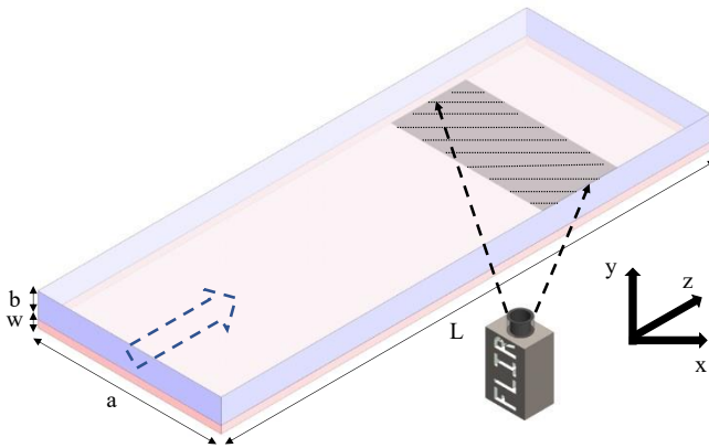
Fig. 3. Minichannel cross-section with the heated foil.
