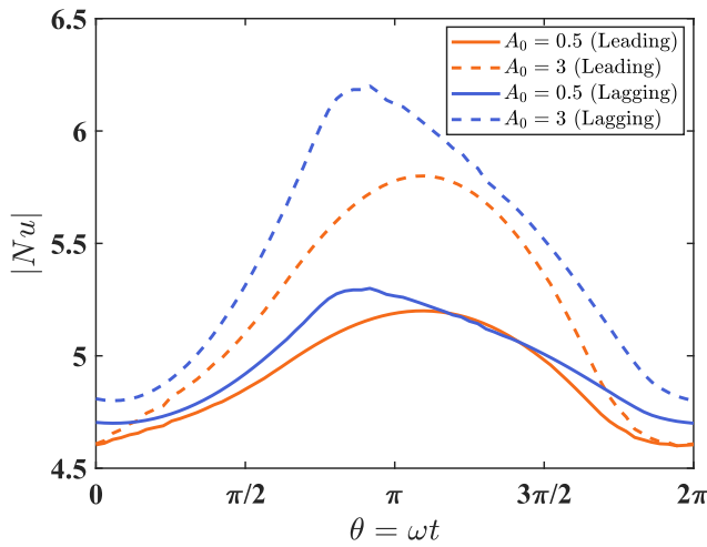
Fig. 9. Temporal variation of the space-averaged instantaneous Nusselt number ( |Nu| ) for leading and lagging asymmetric sinusoidal waveforms for Wo = 2.5 with varying A_0 . For reference, the steady flow Nu_s = 5.08 .
