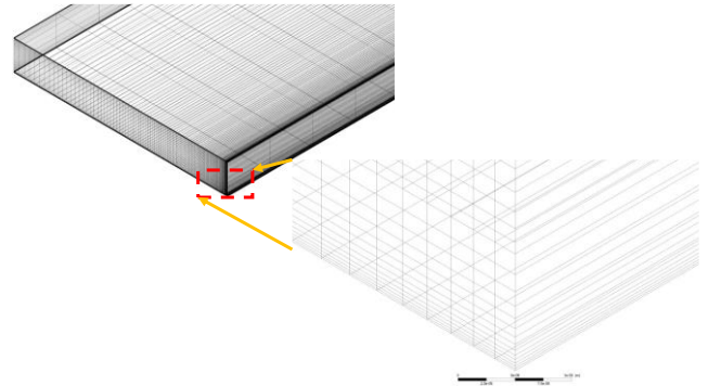
Fig. 5. A two-staged 3D isometric view of the mesh, inclusive of solid and fluid domains.
