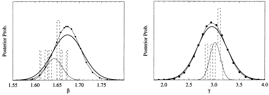
Figure 6. The expected probability distribution of the model parameters \beta and \gamma (heavy line) for model D. The dashed histogram and Gaussian (thin line) show how the measured value varies for different sets of data. The dash-dotted line shows the uncertainty in the parameter because the data are limited. These are combined to give the final distribution (bold). See Section 4.2 for mode details.
