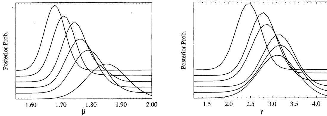
Figure 9. The expected probability distribution of the population parameters for model D. The top curve is for all data, each lower curve is for data remaining when the column density completeness limits are progressively increased by \Delta \log(N) = 0.1 .
