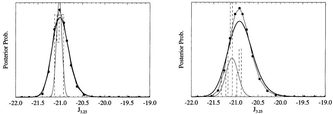
Figure 7. The expected probability distribution of the log background flux at z = 3.25 (heavy line) for models B (left) and D. The uncertainty from the small number of lines near the quasar (line with points) is significantly larger than that from uncertainties in column densities or quasar properties (thin curve). See Section 4.2 for a full description of the plot.
