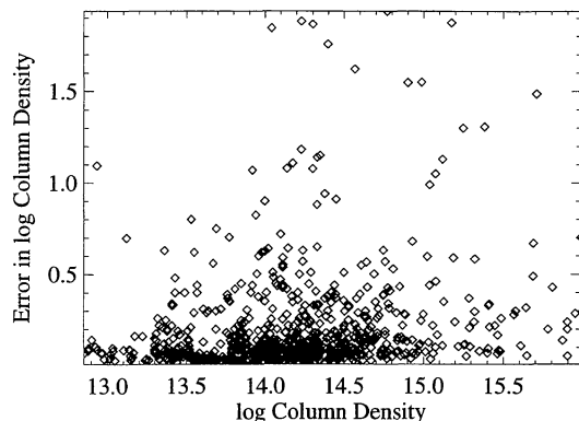
Figure 1. The distribution of errors in column density.
