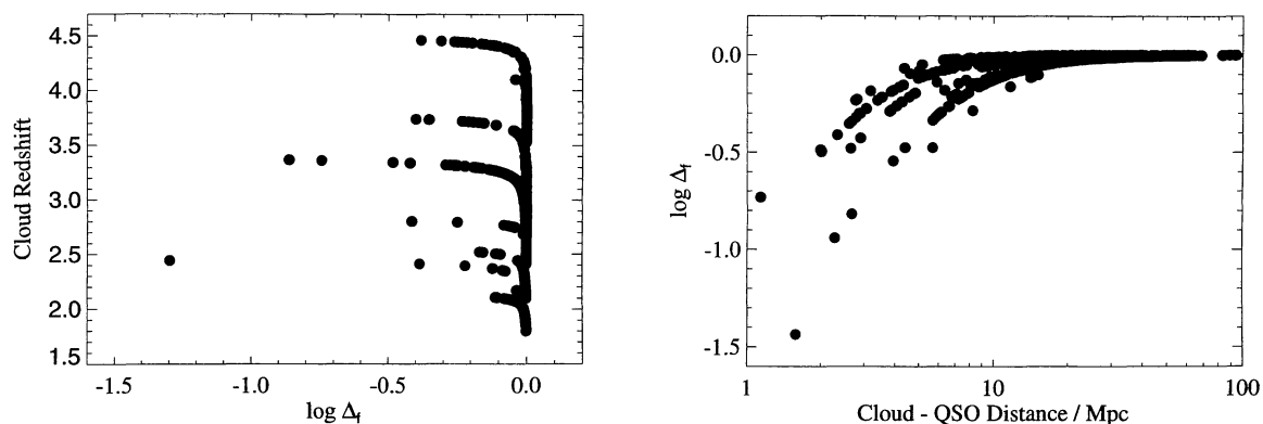
Figure 11. On the left, absorber redshifts are plotted against \Delta_F . On the right \Delta_F is plotted against the distance between cloud and quasar. Note that the correction for the flux of the quasar, and hence the upper limit to the estimate of the background, is significant for only a small fraction of the clouds.
