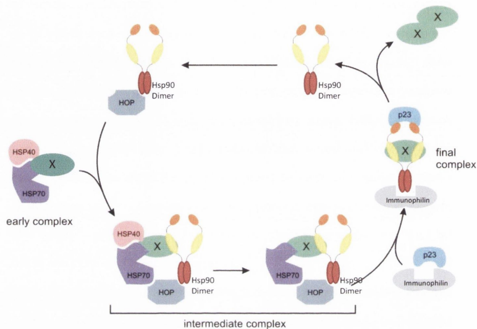
Figure 8: Steroid receptor assembly by the Hsp/immunophilin machinery. Four proteins, Hsp90, p60/Hop, Hsp70 and Hsp40, form a foldosome complex that associates with the stripped, non-steroid-binding state of the glucocorticoid receptor (X) in an ATP/Mg 2+ -dependent and K + -dependent manner to assemble a X-Hsp90-p60-Hsp70-Hsp40 heterocomplex with a steroid-binding site (intermediate complex). p23 is not a component of the native foldosome, but it associates with the assembly intermediate formed with purified proteins as well as with native glucocorticoid receptor-Hsp90 heterocomplexes isolated from cells. In both cases, p23 binding is reversible, does not require ATP and stabilises the complex. Immunophilins such as FKBP52, CyP-40 or the immunophilin-like PP5 bind to Hsp90 via tetratricopeptide repeat (TPR) domains. Because Hop and immunophilins bind to the same TPR acceptor site on Hsp90, immunophilins cannot bind until Hop has dissociated from this site. Immunophilins and p23 binding result in formation of the final complex, whereupon the glucocorticoid receptor is correctly folded and p23, immunophilins and the folded receptor disassociate from the Hsp90 dimer.
