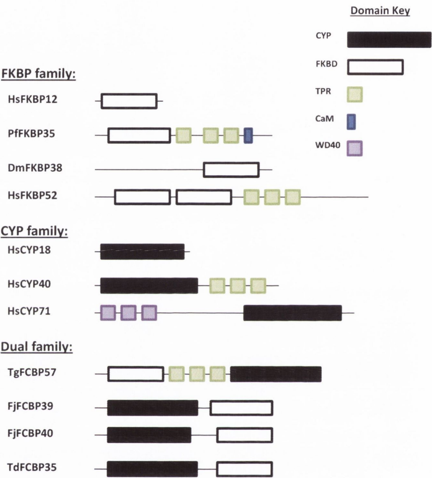
Figure 7: Representative domain arrangements of immunophilins: FKBP, CYP and dual family immunophilins. CYP = cyclophilin domain, FKBD = FK506-binding domain, CaM = putative calmodulin binding domain, WD40 = 40aa Trp/Asp containing \beta -propellor repeat domain, TPR = tetratricopeptide repeat domain, Hs = Homo Sapiens , Pf = Plasmodium falciparum , Dm = Drosophila melanogaster , Tg = Toxoplasma gondii , Fj = Flavobacterium johnsonii , Td = Treponema denticola
