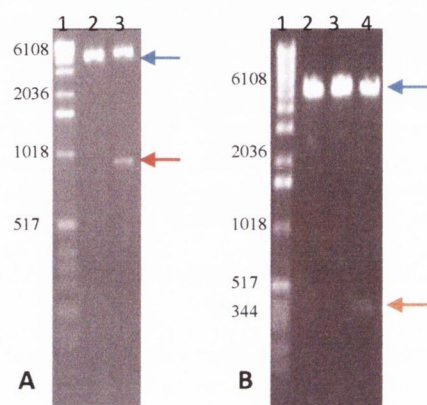
Figure 14: Analysis of pLexA-N bait plasmid constructs. Plasmid isolated from transformant colonies was subjected to EcoRI and PstI digestion, run through a 1% agarose gel and stained with ethidium bromide. (A) Lane 1, Molecular weight marker (MW in bp). Lane 2, ~0.2 \mu g unligated pLexA-N plasmid. Lane 3, ~0.2 \mu g pLexA-N ligated with PffFKBP35 PCR product. Blue arrow: band at ~5600 bp corresponding to pLexA-N. Red arrow: band at ~900 bp corresponding to PffFKBP35 PCR product. (B) Lane 1, Molecular weight marker (molecular weight in bp). Lanes 2+3, ~0.2 \mu g unligated pLexA-N plasmid. Lane 4, ~0.2 \mu g pLexA-N ligated with FKBP-domain PCR product. Blue arrow: band at ~5600 bp corresponding to pLexA-N. Orange arrow: band at ~380 bp corresponding to FKBP-domain PCR product.
