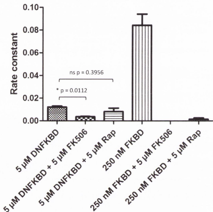
Figure 34: Rate constants of the PPIase activity of FKBD-His 6 and ΔNFKBD-His 6 . The rate constants for FKBD and ΔNFKBD, in the presence or absence of ligands, were determined by calculating the natural logarithm of the remaining substrate (by the formula (A_{\text{max}} - A_{390})/0.0133 = \text{cis remaining [in } \mu\text{M}] ) vs. time and taking the slope of the resulting curve.
