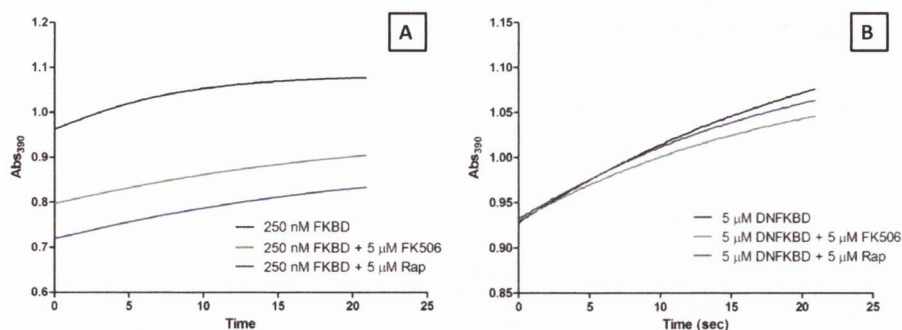
Figure 33: PPIase activity of FKBD-His 6 (FKBD) and ΔNFKBD-His 6 (DNFKBD). FKBD and DNFKBD were used in the assay at 250 nM and 5 μM respectively, either on their own or in the presence of 5 μM FK506 or Rap. Representative curves show increase in absorbance over time.
