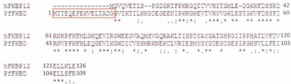
Figure 27: Sequence alignment of human FKBP12 with PffKBD. The red box indicates 15 AA N-terminal extension. Identical residues are indicated with an asterisk, a colon indicates conservation between groups of strongly similar properties and a full stop indicates conservation between groups of weakly similar properties.
