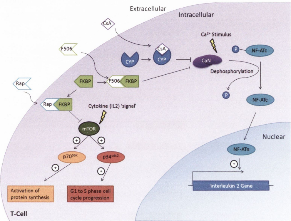
Figure 6: Schematic of the immunosuppressive action of CsA, FK506 and Rap. Cyclosporin A and FK506 bind to cyclophilin (CYP) and FK506-binding protein (FKBP) respectively. These complexes inhibit the dephosphorylation activity of calcineurin (CaN). CaN is unable to dephosphorylate the cytosolic form of nuclear factor of activated T-cells (NF-ATc), in this form NF-ATc is unable to translocate to the nucleus (NF-ATn) where it would normally activate important genes in T-cell proliferation. Rapamycin binds FK506 and this complex inhibits mechanistic target of rapamycin (mTOR) which results in inhibition of T- and B- cell proliferation by inhibiting their response to interleukin 2 (IL-2).
