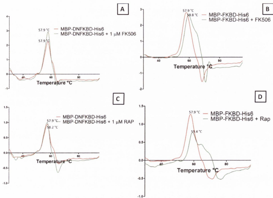
Figure 32: Thermal stability shift assay, showing A. 1 μM MBP-ΔNFKBD-His 6 (red) and 1 μM MBP-ΔNFKBD-His 6 with 1 μM FK506 (green). B. 1 μM MBP-FKBD-His 6 (red) and 1 μM MBP-FKBD-His 6 with 1 μM FK506 (green). C. 1 μM MBP-ΔNFKBD-His 6 (red) and 1 μM MBP-ΔNFKBD-His 6 with 1 μM rapamycin (green). D. 1 μM MBP-FKBD-His 6 (red) and 1 μM MBP-FKBD-His 6 with 1 μM rapamycin (green).
