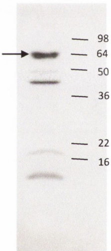
Figure 17: Western blot of ~100 µg crude parasite lysate separated by SDS-12.5% PAGE, transferred to PVDF membrane and probed with anti-Hsp70. The black arrow indicates a band at ~70 kDa; numbers indicate molecular weight marker size in kDa. Lower bands may be the result of protein breakdown in the sample.
