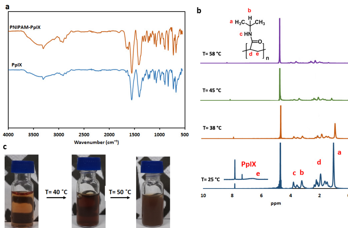
Figure 2. (a) FT-IR spectra of protoporphyrin IX and poly N -isopropylacrylamide-protoporphyrin IX hydrogel; (b) 600 MHz 1 H NMR spectra of PpIX-PNIPAM nanohydrogel in D 2 O at different temperatures; (c) pictorial illustration of the LCST type phase transition of the PpIX-PNIPAM nanohydrogel at 40 °C and 50 °C.
