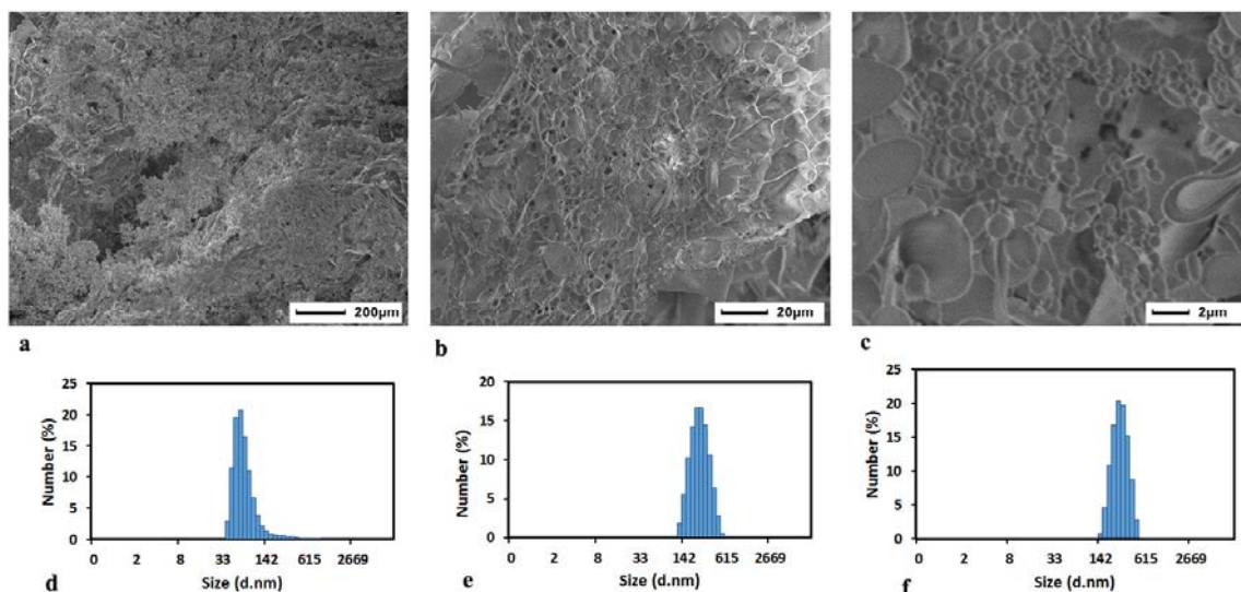
Figure 4. (a, b, c) SEM images of PpIX-PNIPAM hydrogels at different magnifications; (d, e, f) hydrodynamic diameter of PpIX-PNIPAM hydrogel with 2%, 3% and 4% PS, respectively, as determined by dynamic light scattering.
