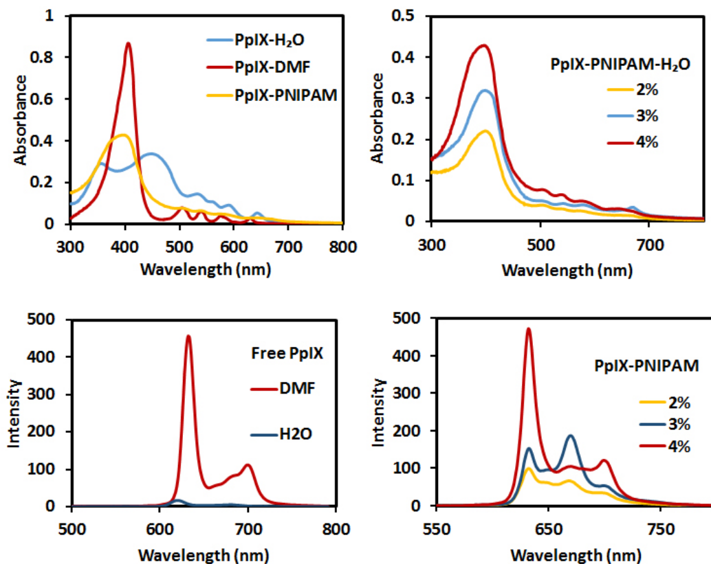
Figure 3. (a) UV-visible spectra of protoporphyrin IX ( 1.5 \times 10^{-4} M) in H 2 O and DMF ( 1.5 \times 10^{-5} M) and PpIX-PNIPAM hydrogel ( 1.5 \times 10^{-5} M) in H 2 O; (b) fluorescence emission spectra of PpIX in DMF and H 2 O ( \lambda_{\text{ex}} = 409 nm); (c) UV-visible absorption spectra of PpIX-PNIPAM hydrogel at different concentrations of protoporphyrin IX in the hydrogel structure (2%, 3%, and 4%) in H 2 O (the concentration of PpIX in 4% PpIX-PNIPAM hydrogel = 1.5 \times 10^{-5} , in 3% = 1.1 \times 10^{-5} , and in 2% = 0.75 \times 10^{-5} M; (d) Fluorescence spectra of PpIX-PNIPAM hydrogel ( \lambda_{\text{ex}} = 409 nm) at different concentrations of protoporphyrin IX in H 2 O.
