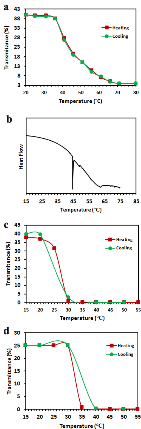
Figure 5. (a) Transmittance versus temperature plots for PpIX-PNIPAM hydrogel ( 1.35 \times 10^{-5} M) in water; (b) DSC thermogram of PpIX-PNIPAM nanohydrogel in water; (c) transmittance
