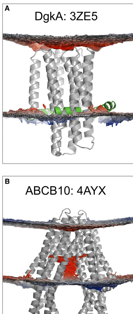
Figure 5. Local Distortions of the Lipid Bilayer
