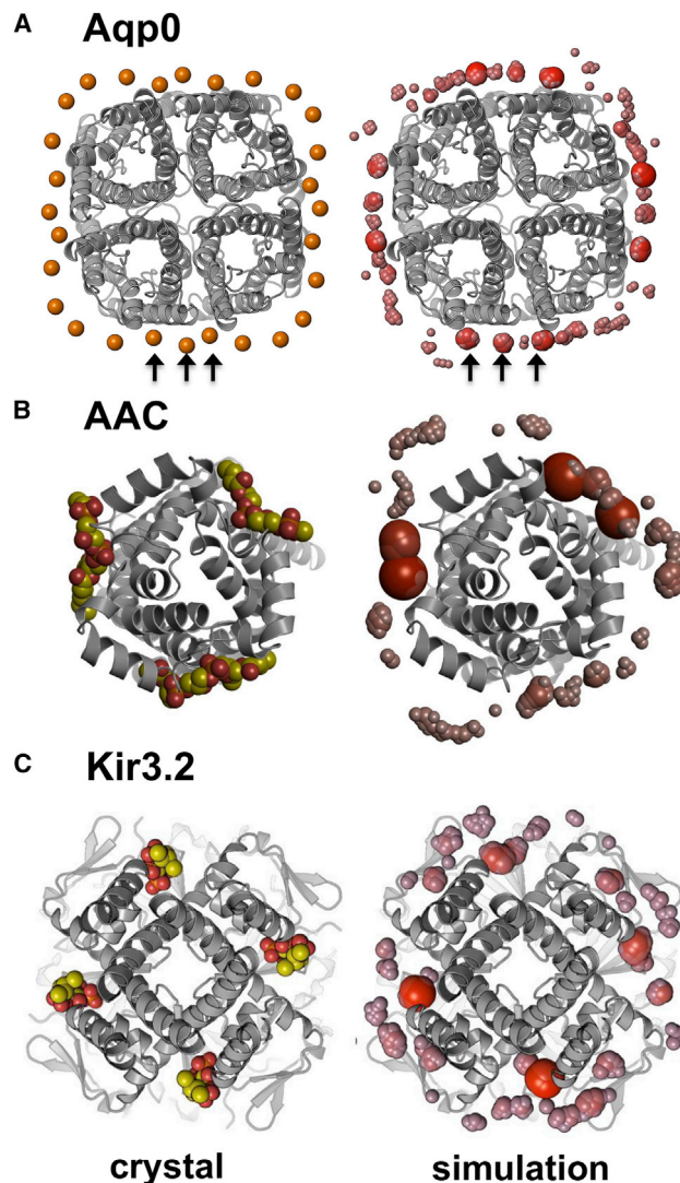
Figure 3. Identifying Lipid Interaction Sites
