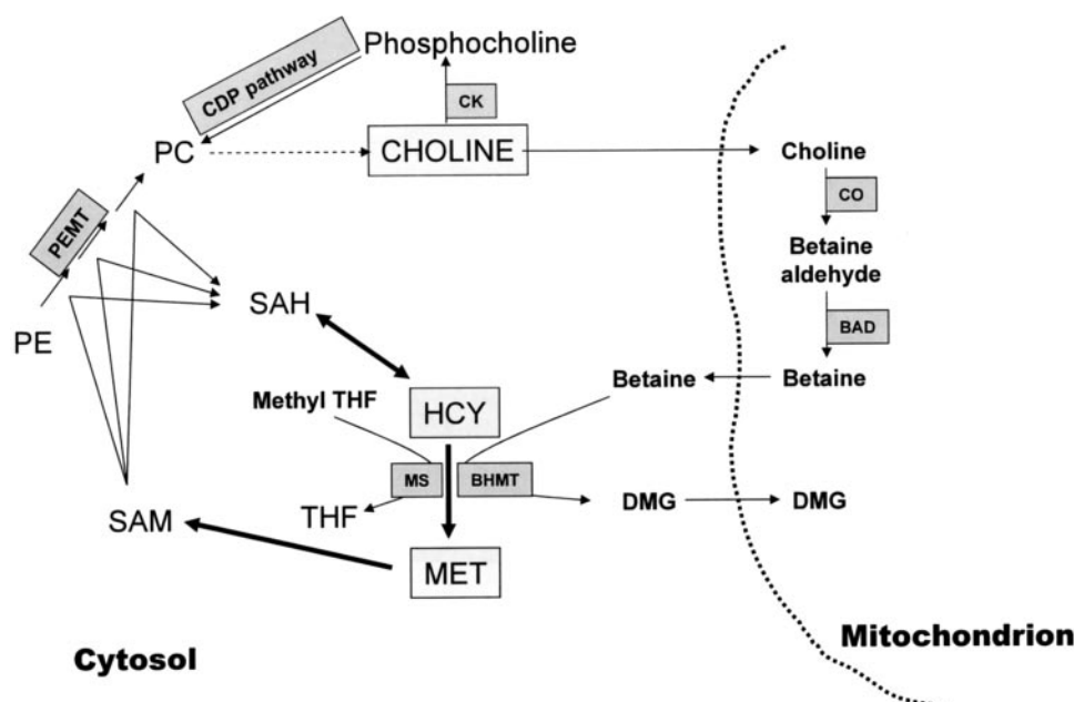
FIGURE 1. Choline and homocysteine interrelations in the liver. BAD, betaine aldehyde dehydrogenase; BHMT, betaine homocysteine methyltransferase; CDP, cytidine diphosphocholine; CK, choline kinase; CO, choline oxidase; DMG, dimethylglycine; HCY, homocysteine; MET, methionine; MS, methionine synthase; PE, phosphatidylethanolamine; PEMT, phosphatidylethanolamine N -methyltransferase; PC, phosphatidylcholine; SAH, S -adenosylhomocysteine; SAM, S -adenosylmethionine; THF, tetrahydrofolate.
