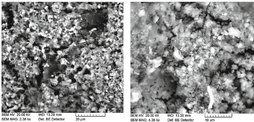
Fig. 6. Hot lime mixed hemp concrete (QL + GGBS mix) under the SEM showing extensive carbonation, with abundant microcrystals of calcium carbonate and some cementing hydrates (needles -left image) and low crystallinity gels (all over).
