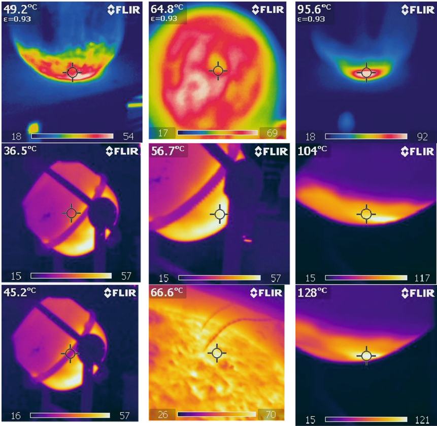
Fig. 4. Evolution of temperature during hot-lime mixing concretes 12 and 13-Table 2.
