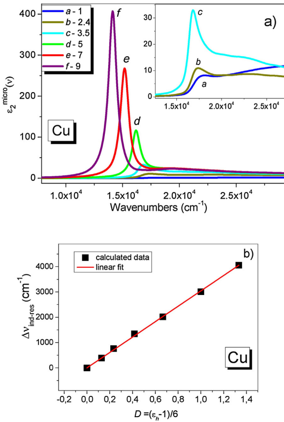
Fig. 1. Dielectric-loss spectra \epsilon_2^{micro}(\nu) of plasmon absorption in spherical particles of Cu in various matrices, calculated in the quasi-static limit from Eqs. (7),(8) with variation of \epsilon_h of the ambient medium: 1 (a), 2.4 (b), 3.5 (c), 5 (d), 7 (e), 9 (f). b) Linear dependence of the inductive-resonant dipole-dipole frequency shift of the absorption maximum by a plasmon in Cu vs dielectric factor D = (\epsilon_h - 1)/6 . The obtained slope, A = \Delta\nu/D , is equal to 3040 cm -1 . The numbers in brackets in caption for Figure a) correspond to the numbers shown beside the relevant curves; the data for curve (a) is multiplied by a factor of 7 and is also shown with curves (b) and (c) in the insert for clarity.
