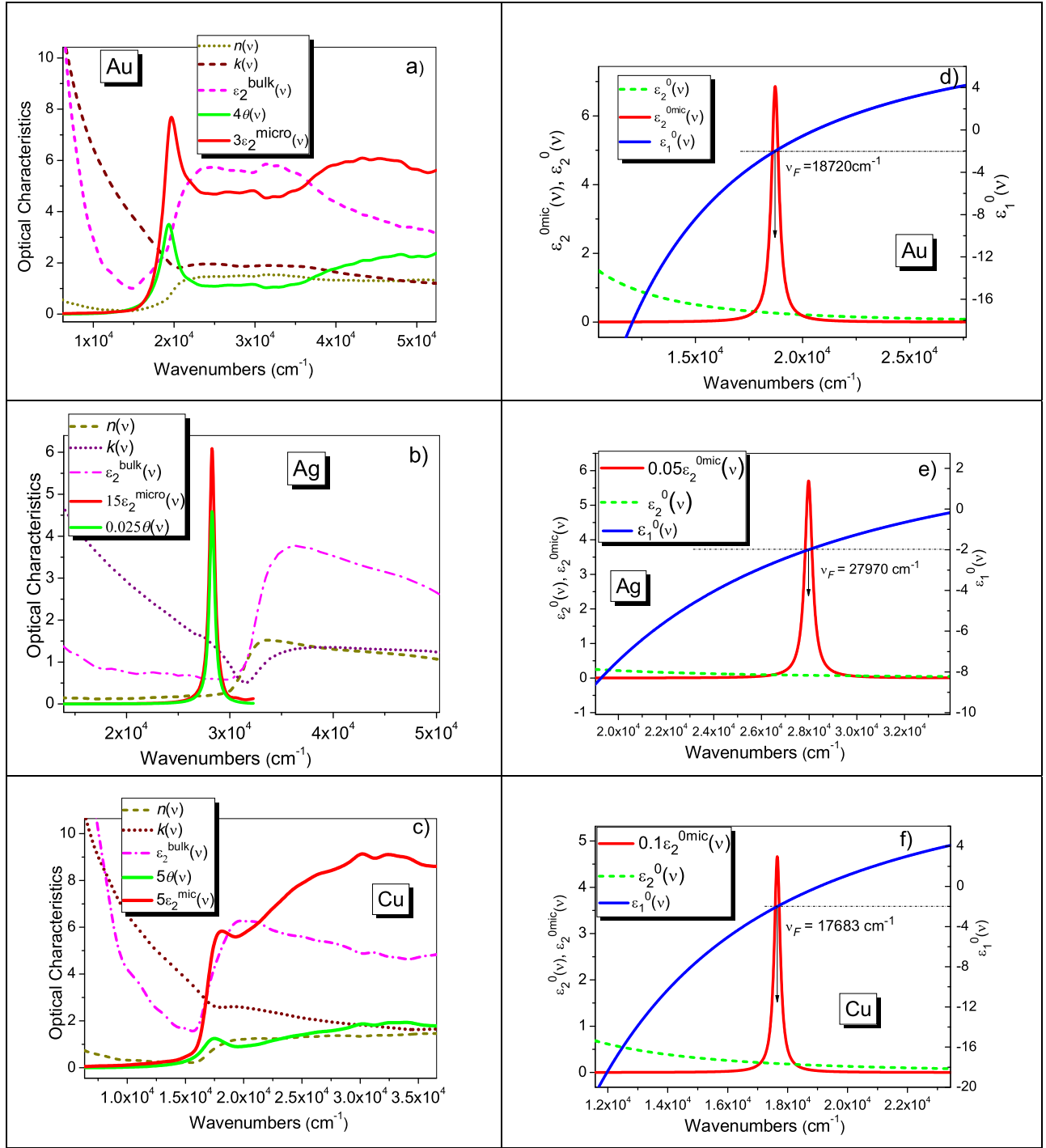
Fig. 2. Experimental and calculated spectra of optical characteristics of noble metals. Calculations of spectra \varepsilon_2^{\text{bulk}}(v) = 2n(v)k(v) , \theta(v) (using Eq. (6a)), and \varepsilon_2^{\text{micro}}(v) (using Eq. (6)) are based on experimental spectra n(v) and k(v) taken from a) Ref. [44] for Au, b) Ref. [45] for Ag and c) Ref. [43] for Cu. The real \varepsilon_1^0(v) and imaginary \varepsilon_2^0(v) parts of dielectric function \varepsilon^{\text{bulk}}(v) , calculated using Eq. (3a) for the bulk metal based on the parameters v_0 , F_0 and \gamma_0 from Ref. [24] for a zero oscillator, and calculated with Eq. (6) using these functions, spectra \varepsilon_2^{\text{omic}}(v) for Au (d), Ag (e) and Cu (f). The peak position of spectrum \varepsilon_2^{\text{omic}}(v) , and the intersection with the spectrum of \varepsilon_1^0(v) , corresponding to Fröhlich's condition \text{Re}\varepsilon(v_F) = -2 , are shown by the number beside each spectrum and by the arrow in figures d), e), and f). For clarity of presentations, some of the spectra are multiplied by the factor shown in the legends.
