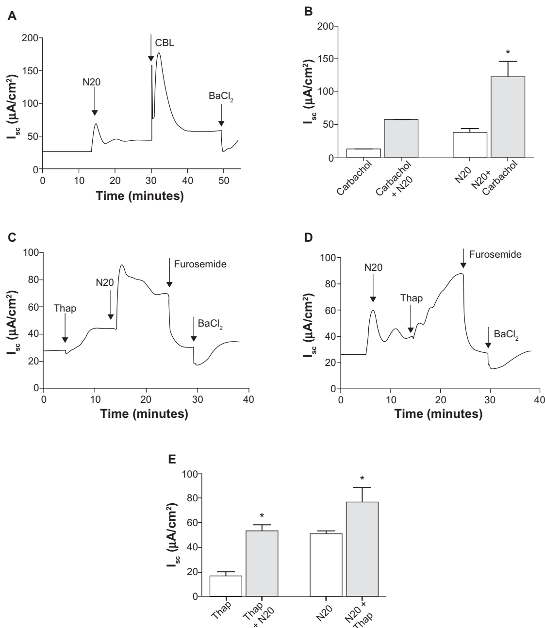
Figure 5 Effect of N20 on calcium-mediated anion secretion in Calu-3 cells. A ) Carbachol-induced I_{sc} (CBL) 100 \mu M basolateral was significantly increased by prestimulation with N20 10 \mu g/mL apical, and BaCl_2 5 mM basolateral as shown inhibited I_{sc} . B ) Statistical analysis of the effects of N20 on I_{sc} in the presence and absence of carbachol. *P < 0.05 ( n = 3 , one-way analysis of variance). C ) Activation of I_{sc} by thapsigargin (Thap) 1 \mu M both sides in Calu-3 cells. N20 further increased I_{sc} in thapsigargin pretreated cells. D ) Thapsigargin-induced I_{sc} was significantly increased by prestimulation with N20. Furosemide 1 mM basolateral and BaCl_2 , as shown in C and D , inhibited I_{sc} responses. E ) Statistical analysis of the effects of N20 on I_{sc} in the presence and absence of thapsigargin. Note: *P < 0.05 ( n = 3 , one-way analysis of variance).
