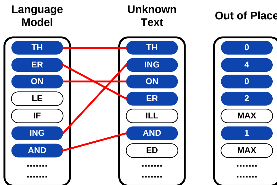
Figure 5-4 Out-of-Place Measure
