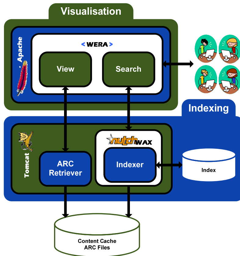
Figure 5-6 Visualisation Architecture
