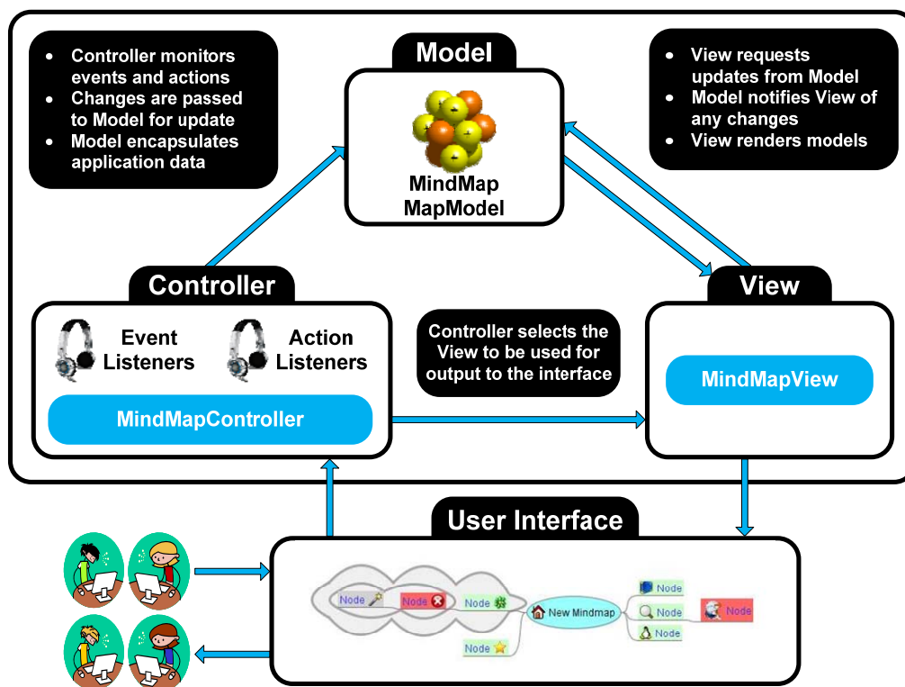
Figure 5-15 Freemind Architecture
