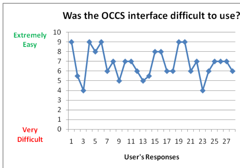
Figure 6-60 Usability Question 5
