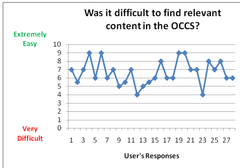
Figure 6-59 Usability Question 4
