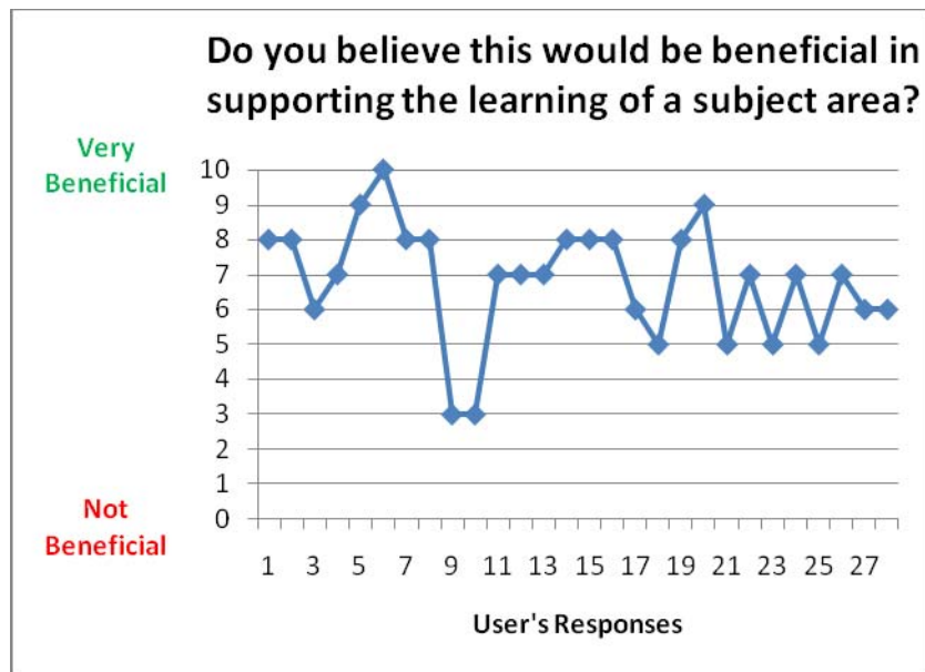
Figure 6-57 Usability Question 2
