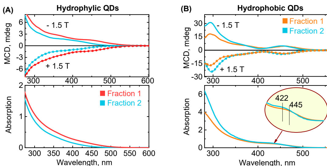
Figure 4. Magnetic circular dichroism (top) and corresponding absorption (bottom) spectra of two fractions of hydrophilic (A) and hydrophobic (B) AIS/ZnS QDs.
