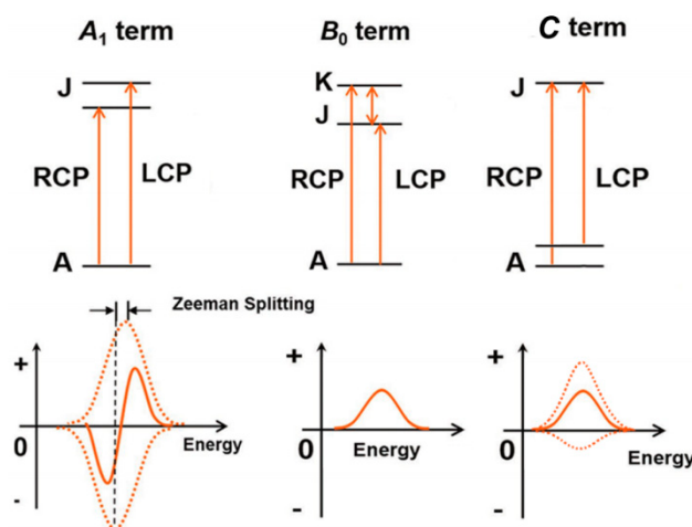
Figure 2. Scheme of band formation in magnetic circular dichroism spectra.
