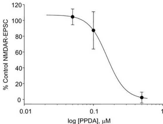
Supplemental Figure 2. Concentration-response curve for PPDA inhibition of extrasynaptic NMDAR-EPSCs. The \text{IC}_{50} value was 0.2 \mu\text{M} ( n = 3-5 ). The extrasynaptic NMDAR-EPSC was measured as the increase in EPSC amplitude above the baseline synaptic current, in the presence of the uptake inhibitor TBOA.
