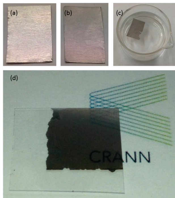
Figure 1. (a) Nickel foil before growth. (b) Nickel foil after growth of MLG film. (c) MLG film floating in water having been etched from growth substrate and transferred. (d) Transparent MLG film transferred to PET sheet.
