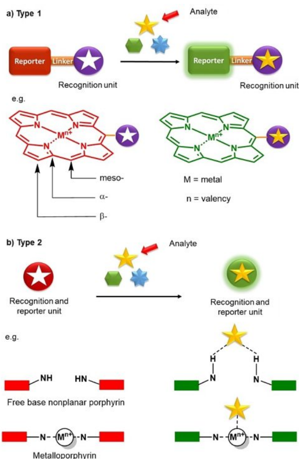
Figure 1. Schematic design of two commonly used organic frame-based sensing platforms. [20] a) Recognition and reporter units separated by a linker, e.g., Cd^{2+} binding reported by Lv et al. to the periphery of H_2-7^{(26)} b) Recognition and reporter function as one unit, e.g., free-base porphyrin o - H_2OET_{NH_2}PP binding pyrophosphate in its inner core reported by Norvaiša et al. [33] or metalloporphyrin Ni^{II}TPP(CN)_4 coordinating CN^- anions to a metal center reported by Kumar et al. [28b]
