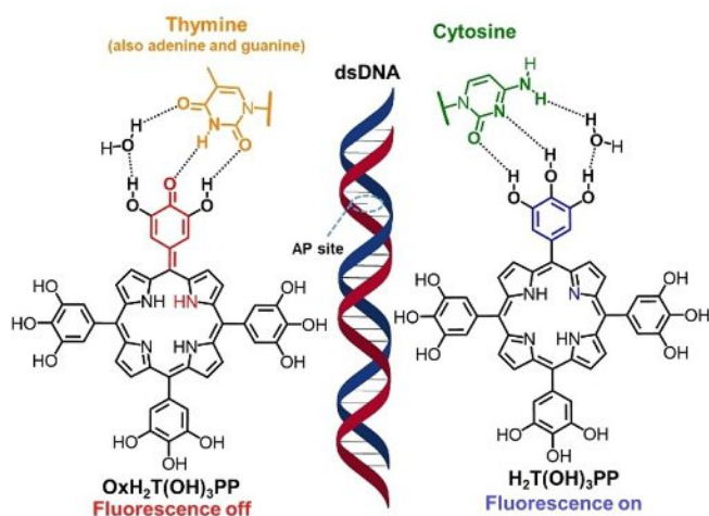
Figure 9. AP site interactions of dsDNA and \text{H}_2\text{T}(\text{OH})_3\text{PP} : fluorescence changes are induced upon interaction with cytosine ("on") and other nucleobases ("off"), respectively. [153]
