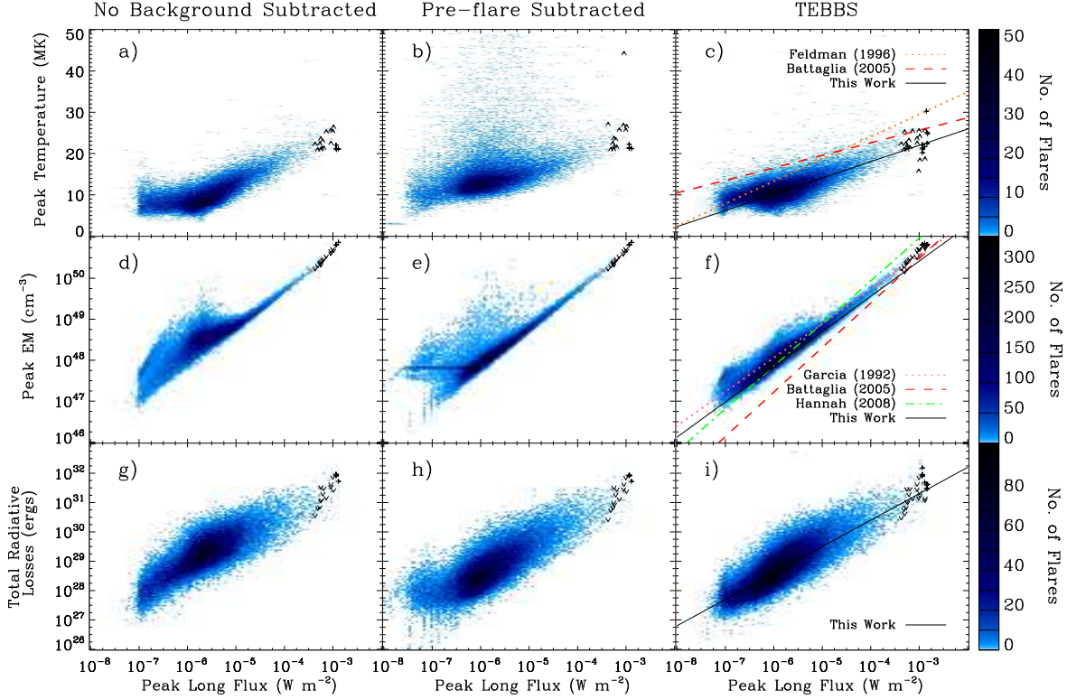
FIG. 8.— Two-dimensional histograms of peak temperature, peak emission measure, and total radiative losses, each as a function of peak long channel flux, derived using various background subtraction techniques for all selected GOES events observed between 1980 and 2007. The data in the left column has not had the background subtracted. The data in the middle column had the pre-flare flux subtracted, while the distributions in the right column have been derived using the TEBBS method. Overplotted on panels c and f are the relationships derived by Garcia & McIntosh (1992, purple dotted line), Feldman et al. (1996b, orange dotted line), Battaglia et al. (2005, red dashed line), and Hannah et al. (2008, green dot-dashed line). The solid black lines show relationships described by Equations 5, 6 and 8. The arrow heads mark events which are upper or lower limits due to saturation of the XRS and point in the direction that the true value would have been located. The crosses mark events which display lower flux limits and derived properties which are neither upper nor lower limits but only rough estimates. This is because their derived properties are functions of the fluxes in both channels which each saturated. See Appendix for a more detailed discussion of the effects of saturation on derived flare plasma properties and the saturation levels of the XRS on the various GOES satellites.
