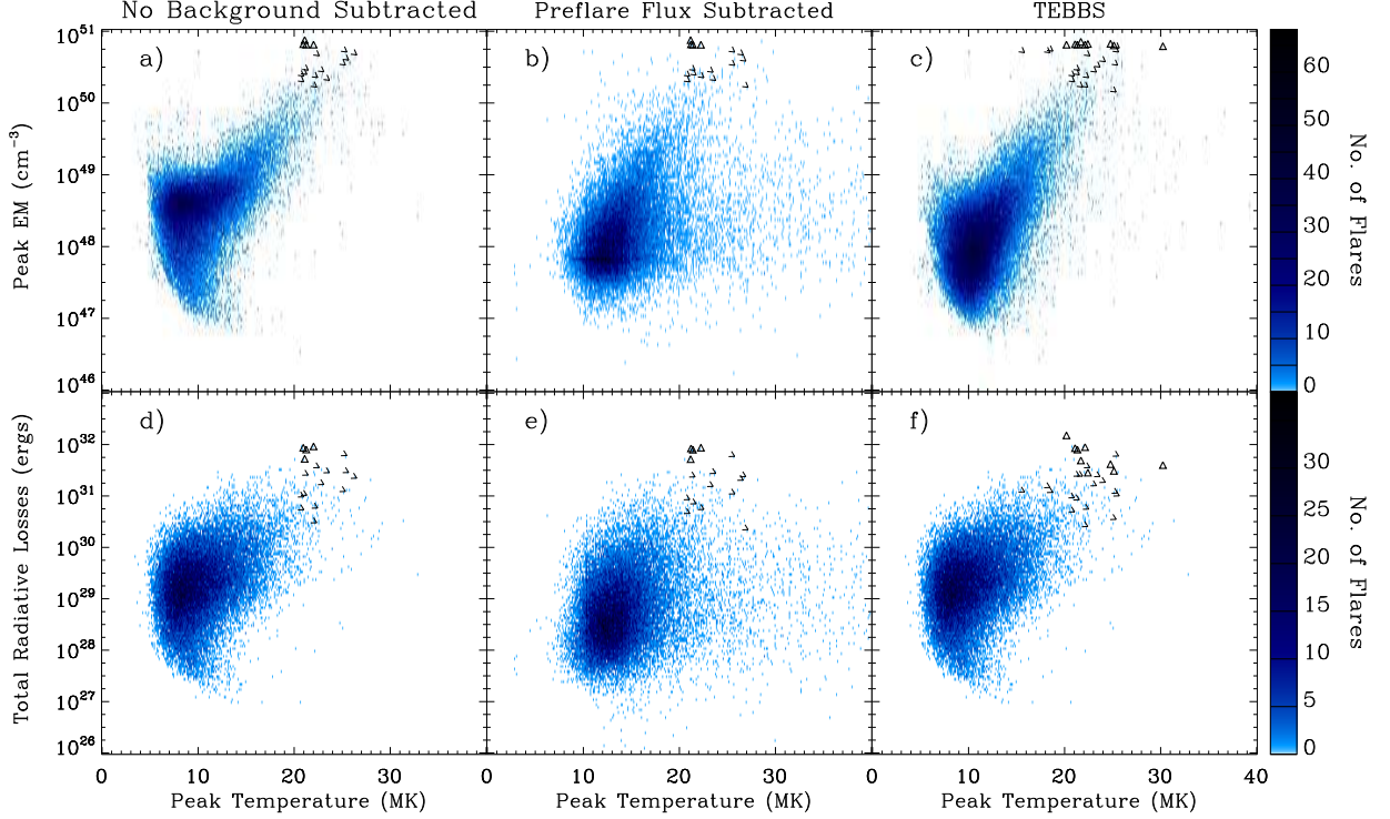
FIG. 9.— Two-dimensional histograms of peak emission measure and total radiative losses as a function of peak temperature for each of the three background subtraction techniques. The arrow heads mark events which are upper or lower limits due to saturation of the XRS and point in the direction that the true value would have been located. The triangles mark events whose values are only rough estimates due to both channels saturating. See Appendix for a more detailed discussion of the effects of saturation on derived flare plasma properties and the saturation levels of the XRS on the various GOES satellites.
