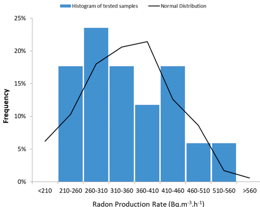
Fig. 12. Distribution of the radon production rates ( Bq.m^{-3}.h^{-1} ) obtained from the analysis of 17 black shale samples.
