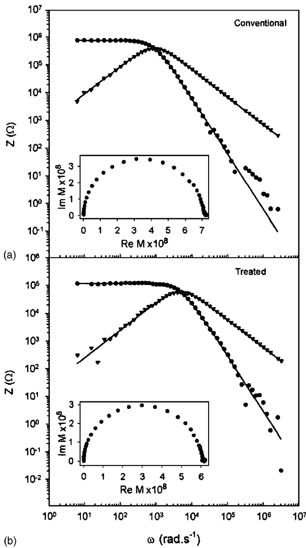
FIG. 4. Re Z (solid circles) and |Im Z| (solid inverted triangles) vs angular frequency, for (a) a conventional and (b) a treated PmPV film. The individual (dotted line) and simultaneous (solid line) fits are also shown. Both devices were prepared using platinum electrodes. The ac bias is 5 mV and the dc bias is 0 V. Both plots have been normalized for film thickness. It is noted that the individual fits are obscured in the plot due to the excellent correlation between the simultaneous fits and the individual fits to Re Z and Im Z . The Cole-Cole plot for the data is shown in the inset.
