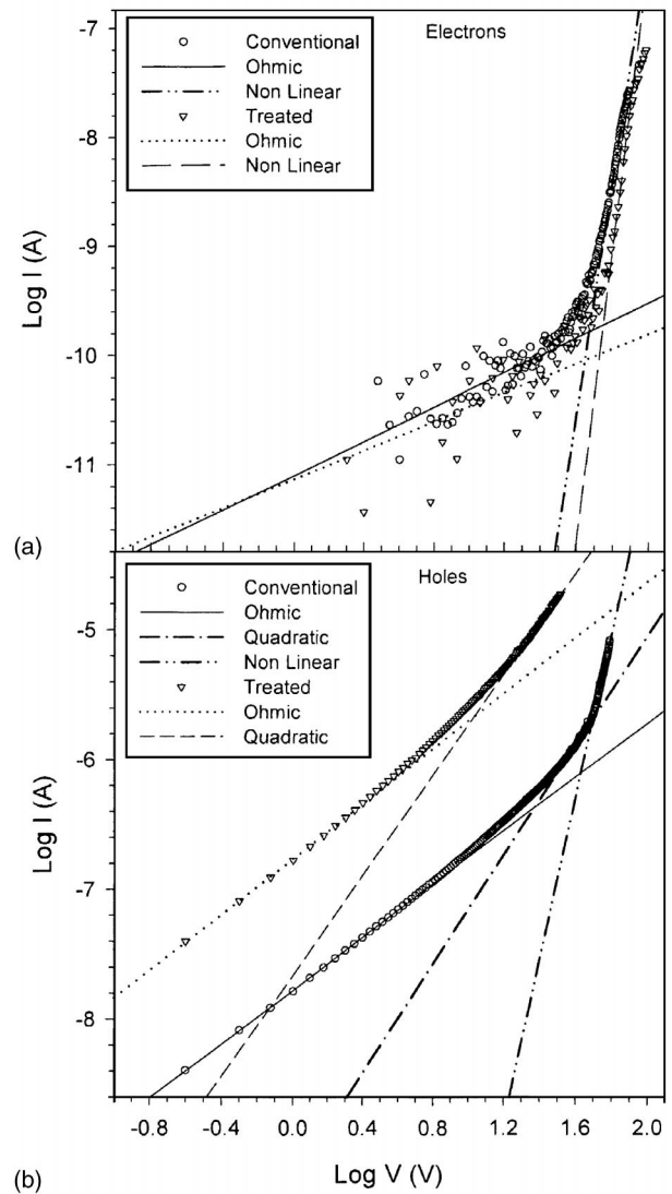
FIG. 5. (a) \log I vs \log V plot for a conventional (open circle) and a treated (open inverted triangle) PmPV film using aluminum electrodes. (b) \log I vs \log V plot for a conventional (open circle) and a treated (open inverted triangle) PmPV film using platinum electrodes. Linear, quadratic, and non-linear fits to the data are shown.
