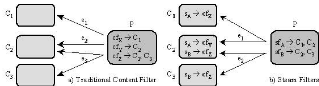
Figure 3. Content vs. STEAM Filters.
