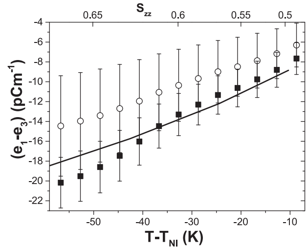
FIG. 2. The experimentally determined value of (e_1 - e_3) at frequencies of 10 Hz ( \blacksquare ) and 1 kHz ( \circ ) as a function of temperature (bottom axis) and order parameter (top axis). The solid line shows values for (e_1 - e_3) calculated using atomistic modelling as a function of order parameter for the molecular axis passing through the carbon atoms of the oxadiazole ring ( S_{zz} ). The measurements of (e_1 - e_3) are assumed to take a negative value, following calculations.
