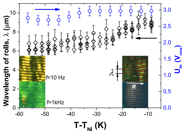
FIG. 1. The temperature dependence of the wavelength ( \diamond ) and threshold voltage ( \circ ) measured at a frequency of 10 Hz for C5-Ph-ODBP-Ph-OC12. The data are presented with respect to the temperature difference from the nematic to isotropic phase transition, T_{NI} . The insets: patterns of the flexodomains between crossed polarizers for T - T_{NI} = -50 K (left) and T - T_{NI} = -15 K (right) for 10 Hz (top) and of longitudinal rolls at 1 kHz (bottom); the images are 60 \mu\text{m} wide.
