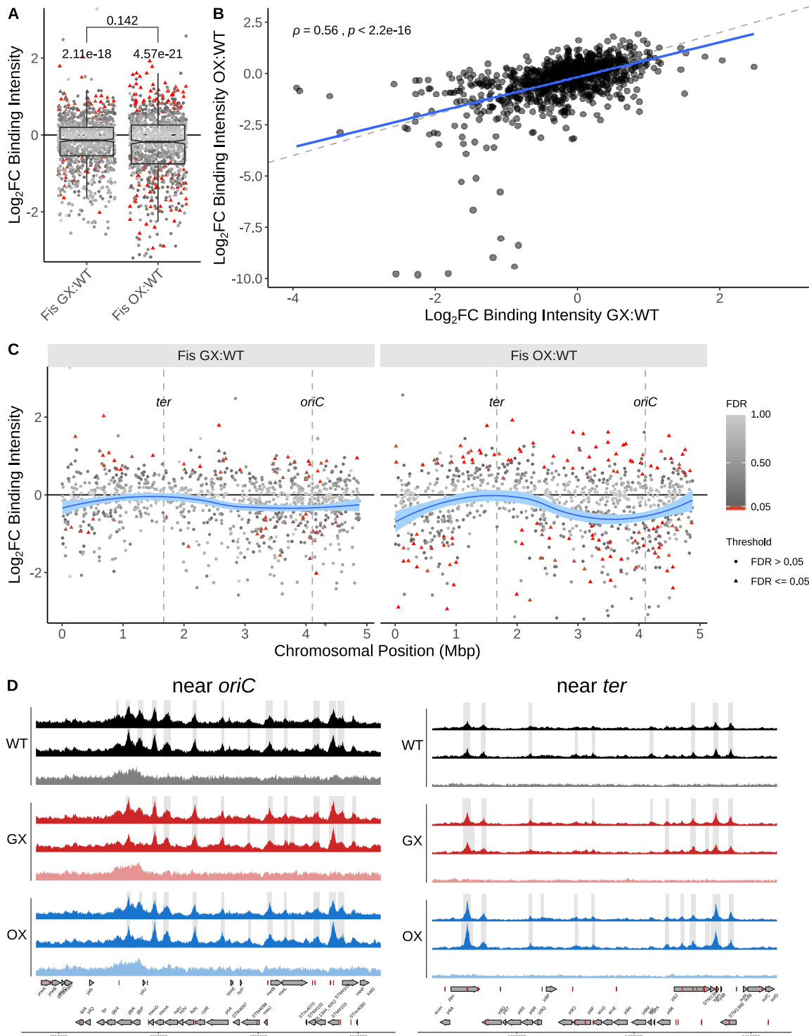
FIG 3 Fis binding changes assayed by ChIP-seq during EE phase. (A) ChIP-seq was used to identify Fis peaks in WT, GX, and OX. The R package DiffBind was then used to determine Log 2 fold changes in binding intensities of Fis in these peaks in the GX and OX strains relative to the wild type. Significant peak intensity changes (FDR < 0.05) are shown as red filled triangles. To determine if the medians of the distributions of Log 2 fold changes in binding intensities differed significantly from 0 (no change in Fis binding relative to WT), the Wilcoxon rank sum test was performed with \mu = 0 ; the P values are displayed above the individual distributions. The difference between the medians of the GX:WT distribution and the OX:WT distribution was not significant with the Wilcoxon rank sum test as shown above the square bracket corresponding to the data from the single-sample tests (using the less conservative Welch's t test here gives a P value of 0.0105). (B) Spearman's correlation of peak intensity changes in the GX in comparison with the OX strain. Dashed line has a slope of 1 and indicates the position where the fold changes in Fis binding intensity in GX would be equal to those in OX. The blue solid line is the regression linear fit to the data. (C) Peak intensity changes along the chromosomal position shown in millions of base pairs. The blue curve shows the local regression peak intensity change calculated using the R locally estimated scatterplot smoothing (LOESS) function.
