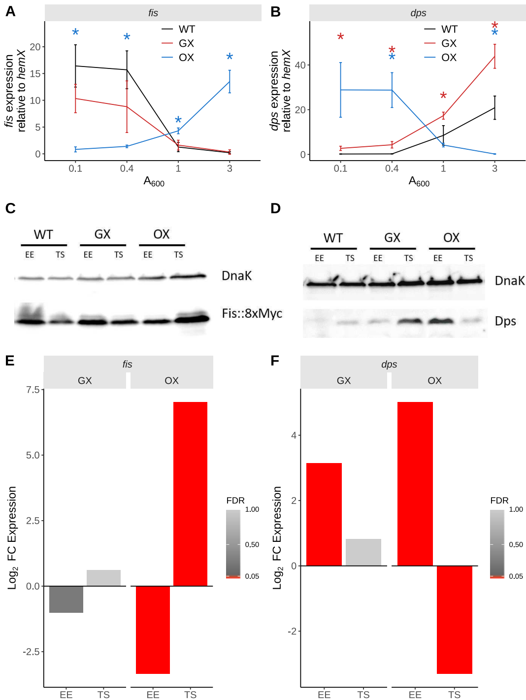
FIG 2 Gene expression changes. (A) Expression of fis transcript during the course of the growth curve assayed using RT-qPCR. Significance was determined relative to the wild type using Welch's t test, and P values were adjusted using the BH method. Adjusted P values are indicated with asterisks (*, P < 0.05; **, P < 0.01; ***, P < 0.001; ****, P < 0.0001). Black, WT; red, GX; blue, OX. (B) Expression of dps transcript during the growth curve. Black, WT; red, GX; blue, OX. (C) Fis protein levels determined by immunoblotting with anti-Fis monoclonal antibody. (D) Dps protein levels determined by immunoblotting with anti-Dps polyclonal serum. (E and F) Expression changes in fis and dps genes determined by RNA-seq in the GX and OX strains at the EE and TS phases of growth. The color bar indicates FDR, and bars representing genes with FDR values of <0.05 are red.
