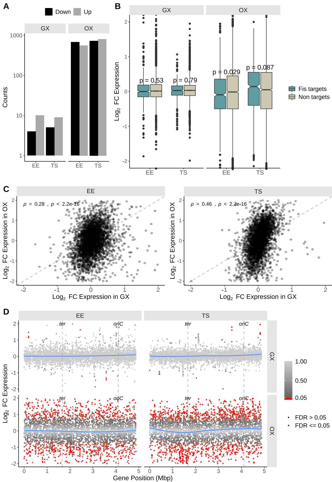
FIG 4 Transcriptomic changes assayed by RNA-seq. (A) Counts of differentially expressed genes. (B) Box plot distribution representations of Log 2 fold change in expression of genes in the GX and OX strains. The genes have been split into two groups based on whether or not they are predicted to be Fis targets. P values obtained using the two-sample Wilcoxon test for the comparison between Fis targets
