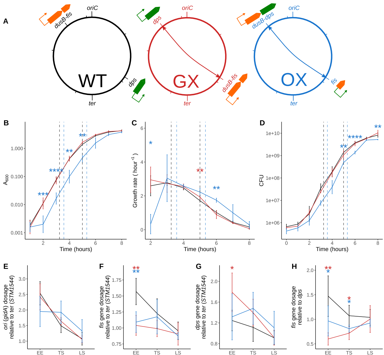
FIG 1 Genomic exchanges of fis and dps transcription units or ORFs. (A) Schematic depicting wild-type (WT) SL1344 strain with the original locations of dusB-fis and dps transcription units shown, the constructed gene exchange (GX) strain with the transcriptional units exchanged, and the ORF exchange (OX) strain with only the fis-dps ORFs exchanged. (B) Optical density-based growth curves showing the impact of these genetic changes on growth. Early exponential (EE), transition to stationary (TS), and late stationary (LS) time points selected for other analyses are shown. Significance was determined relative to the wild type using Welch's t test, and P values were adjusted using the Benjamini Hochberg (BH) method. Adjusted P values are indicated with asterisks (*, P < 0.05 ; **, P < 0.01 ; ***, P < 0.001 ; ****, P < 0.0001 ). (C) Growth rate curve derived from the OD-based growth curves. (D) CFU-based growth curves. (E) Origin-to-terminus gradients in these strains during the course of the growth curve analysis calculated by assaying the abundance of gidA ( oriC proximal gene) DNA and STM1544 ( ter proximal gene) DNA using qPCR. The late stationary (LS) phase is the 24-h time point in the growth curve not shown in the earlier plots. (F) Dosages of the fis gene relative to the terminus during the course of the growth curve analysis. (G) Dosages of the dps gene relative to the terminus. (H) Dosages of the fis gene relative to dps analyzed to understand the impact of the gene position swap.
