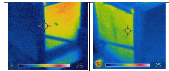
Fig. 4: Infrared thermography showing the absence of thermal bridges and the temperature differential between the hotter, un-rendered [left] at c. 18.2^\circ\text{C} and the cooler, rendered brick wall [right] at 13.9^\circ\text{C} .
