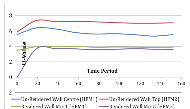
Fig. 3: Thermal transmittance of one of the brick walls over time.
