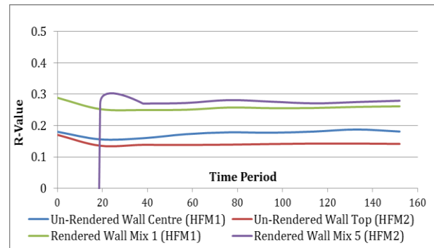
Fig. 2: Thermal resistance of one of the brick walls over time.
