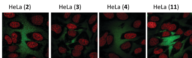
Fig. 3 Incubation of compounds 2–4 and 11 (0.1 mM) for 3 h in HeLa cells. Compounds were excited with a high power laser.
