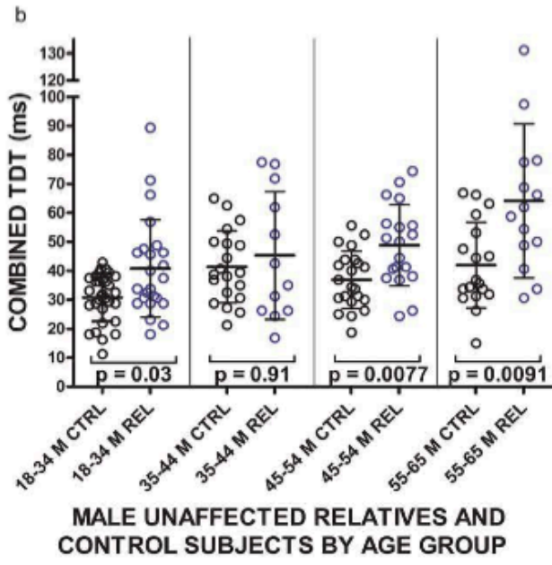
FIG. 1. (a,b) Combined temporal discrimination thresholds (TDTs) (in milliseconds) are illustrated for unaffected first-degree relatives of patients with cervical dystonia compared with the TDTs for healthy control participants according to age group and gender. Shown are the results for (a) female controls (F CTRL) (black circles) and relatives (F REL) (red circles) and for (b) male controls (M CTRL) (black circles) and relatives (M REL) (blue circles). The solid horizontal bars and error bars in the columns represent the mean TDT and standard deviation for each group, respectively. P values refer to a Mann-Whitney comparison of medians.
