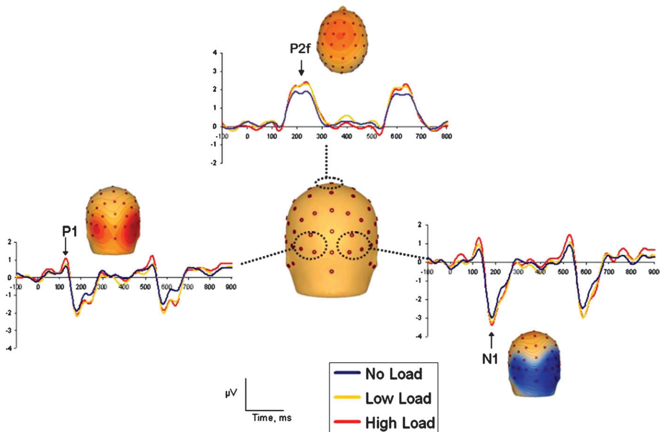
Figure 6. Grand average ERP time locked to the onset of a central stimulus when no peripheral target was presented. Central stimuli were presented every 400 ms; thus, in this 1000 ms segment, there are 2 instances of the classic P1/N1 visual-evoked potential. Accompanying scalp topographies demonstrate the occipital focus for both of these components. The amplitude of both the P1 and the N1 increased as a function of attentional load suggesting increased visual attention to central stimuli. An additional frontocentral component (P2f) also increased in amplitude with central load.
