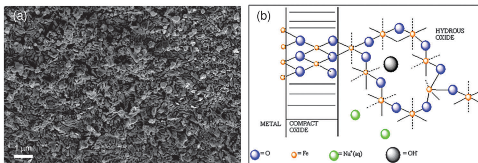
Fig. 3 (a) SEM image of a hydrous oxide covered iron electrode. The film was prepared in 1.0 M NaOH for 120 cycles between -1.30 V and 0.75 V at a sweep rate of 400 \text{mV s}^{-1} . (b) Schematic representation of the Burke-O'Sullivan Duplex Layer Model of the oxide/solution interface.
