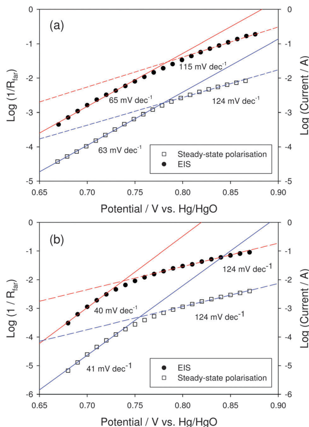
Fig. 28 Tafel plots generated from EIS and Steady-state polarisation data recorded in 1.0 M NaOH for (a) Type A and (b) Type B 120 cycled hydrous oxide films.
