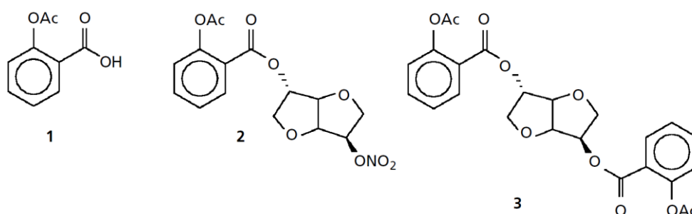
Figure 1 Chemical structures of aspirin (1), ISMNA (2) and ISDA (3).
