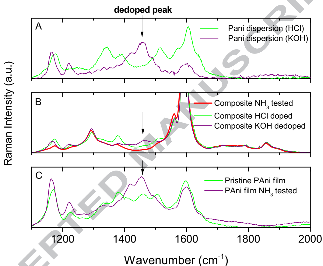
Fig. 5: Raman Spectra of A) PANi dispersions B) Composite Films C) supported PANi films.
