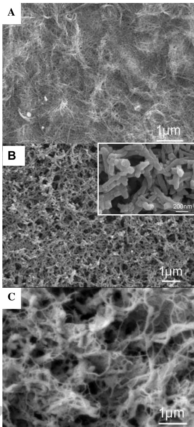
Fig. 2: FESEM of A) CNT buckypaper, B) PANi nanofibers, C) surface of composite material.
