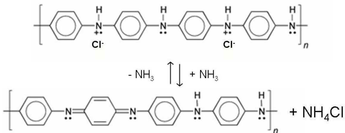
Fig. SI2: PAni dedoping by \text{NH}_3 .
