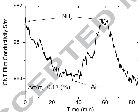
Fig. SI3 Conductivity change of CNT only film to cycled exposure to 10ppm \text{NH}_3 and air.
