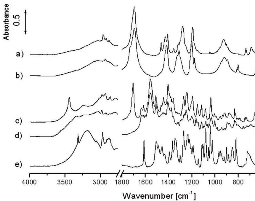
Fig. 7. FTIR spectra of: a) adipic acid, b) succinic acid, c) SA, d) SSU, e) SB. 80x64mm (266 x 266 DPI)
