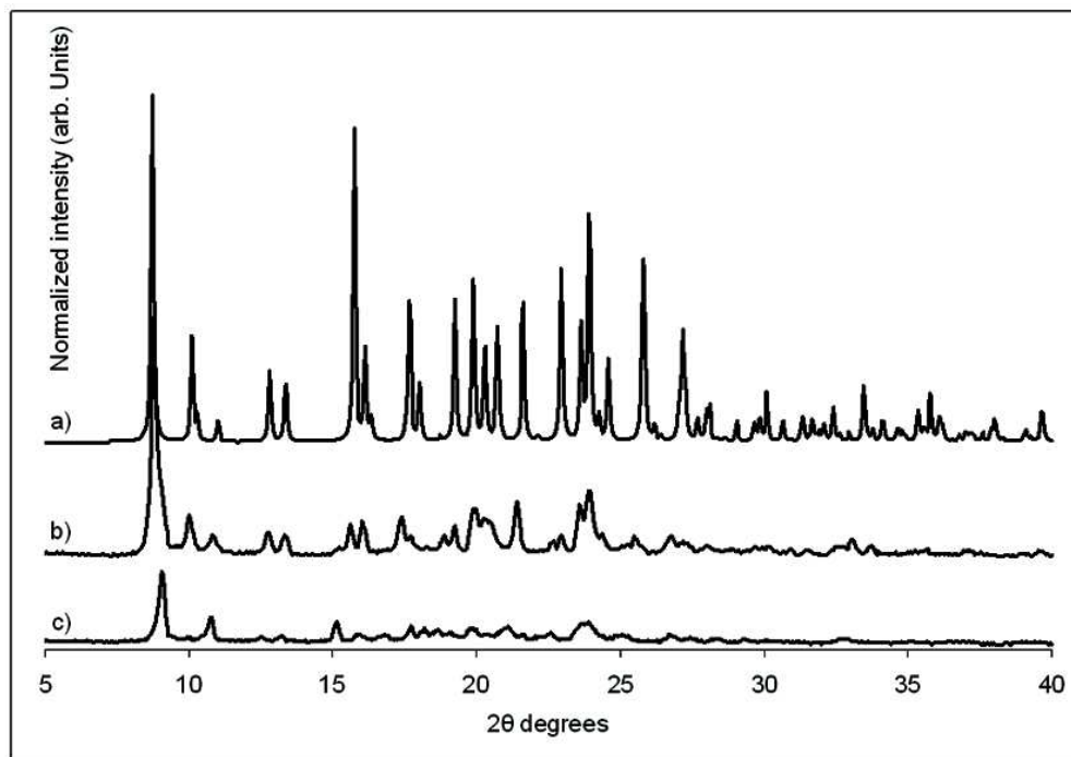
Fig. 5. Comparison of PXRD patterns: a) SSU.MeOH theoretical pattern, b) SSU.MeOH experimental diffractogram and c) SSU experimental diffractogram. 80x56mm (266 x 266 DPI)
