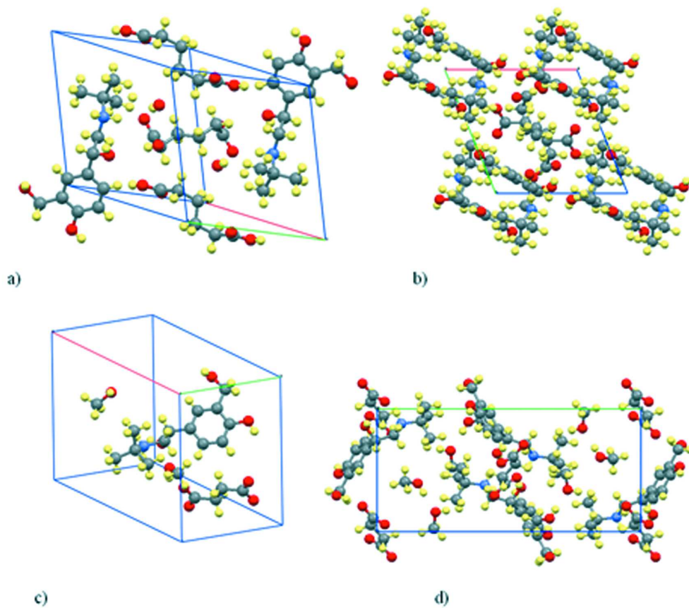
Fig. 2. a) unit cell of SA, b) extended packing diagram of SA along c axis, c) unit cell of SSU.MeOH, d) extended packing diagram of SSU.MeOH along b axis. 165x143mm (266 x 266 DPI)
