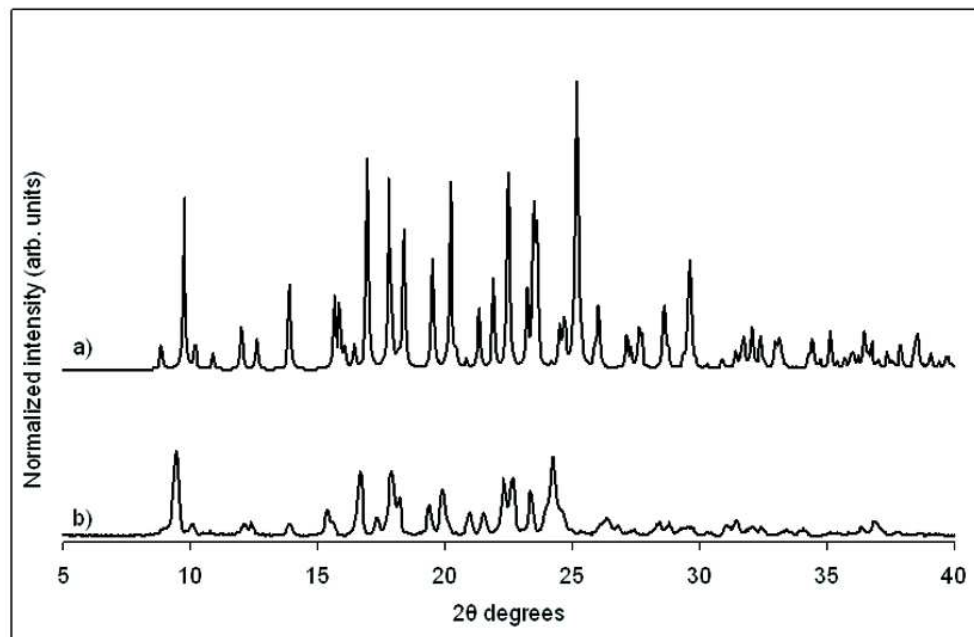
Fig. 4. Comparison of SA PXR D patterns: a) theoretical pattern, b) experimental diffractogram. 80x53mm (266 x 266 DPI)
