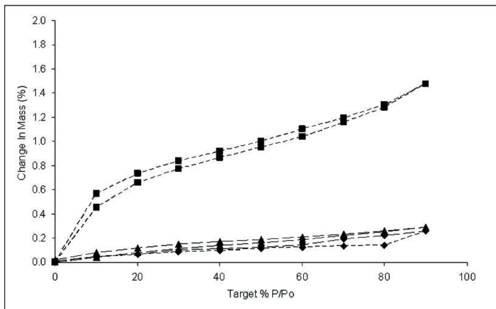
Fig. 8. Dynamic Vapor Sorption of: SA (squares), b) SSU (triangles), c) SS (diamonds). 80x50mm (266 x 266 DPI)
