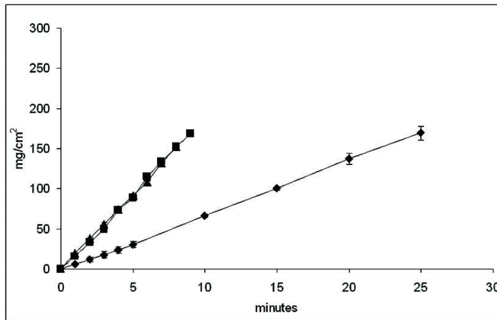
Fig. 10. Intrinsic dissolution profiles of SA (diamonds) and SSU (squares) and SS (triangles). 80x52mm (266 x 266 DPI)
