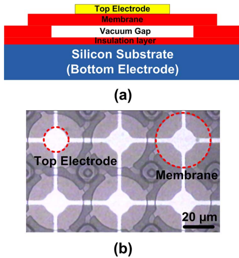
FIG. 1. (Color online) (a) Schematic of a single membrane of a cMUT device. (b) Optical image of a portion of a cMUT array element.
