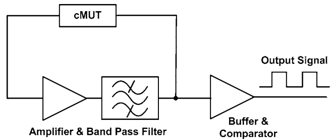
FIG. 3. Simplified block diagram of the oscillator circuit.
