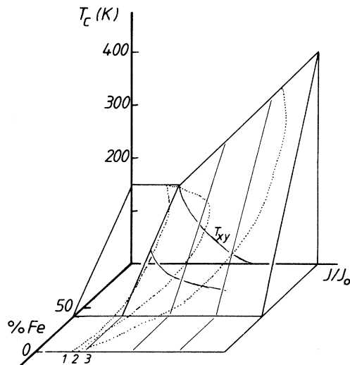
FIG. 8. Magnetic phase diagram for \alpha -Fe x M 100-x alloys (schematic) based on the model of Gabay and Toulouse (Ref. 22). Track 1 represents the path taken for M = \text{Sc} or \text{Y} . Track 2 represents the path taken for M = \text{Zr} or \text{Hf} . Track 3 is for any of the hydrogenated alloys.
