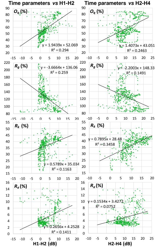
Figure 1: Data for time domain parameters O_q , R_g , R_k and R_a vs H1-H2 and H2-H4.
