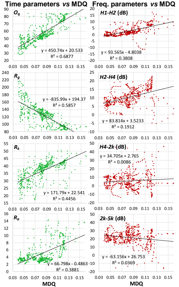
Figure 2: MDQ values compared to time (left) and frequency (right) domain measures.
