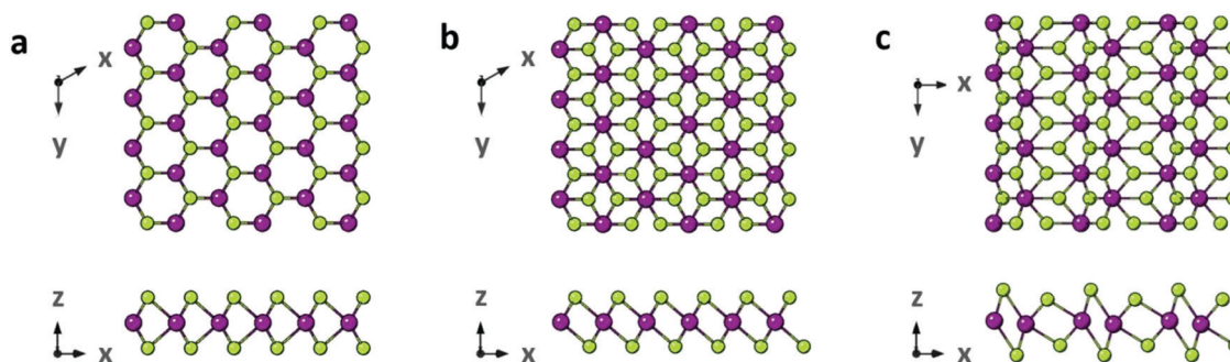
Fig. 5 Structural polymorphs of WSe 2 . (a) 2H WSe 2 (space group P6_3/mmc ). (b) 1T WSe 2 (space group P\bar{3}m1 ). (c) 1T' WSe 2 (space group P2_1/m ). Reproduced from ref. 33.
