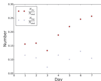
Fig. 8 Plot showing the variation of the ratios N_{\text{fcc}}/N_{\text{total}} and N_{\text{hcp}}/N_{\text{total}} . The fraction of hcp ordering remains roughly constant, while the fraction of fcc ordering rises.
