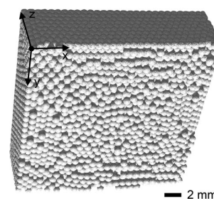
Fig. 1 Visualisation of the gas phase of the sample, showing the bottom of the sample, i.e. the foam–liquid interface. Gravity acts perpendicular to this surface in the z direction. Around the boundary of the foam sample, regions of hexagonal close-packed ordering are seen to occur, while the central region appears disordered.
