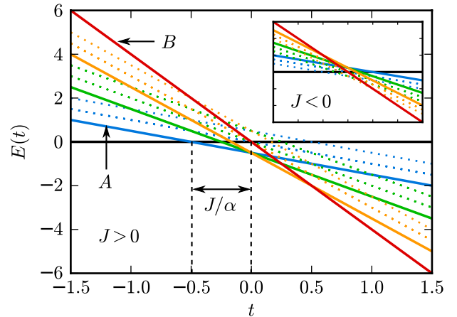
FIG. 1 (color online). Time-dependent eigenenergies of the one-dimensional chain, Eq. (4), with g = 0 , J = \frac{1}{2} and N = 4 sites. Different colors indicate bands corresponding to different values for the occupation n of the two-level systems. Bold lines show the states in each band with maximum S^2 , which are coupled together when the pump is spatially uniform. Dotted lines are other eigenstates of the system, which have different values of S^2 . The vertical dashed lines show the separation in time between the crossing of the n = 0 band with the n = 1 (A) and n = N (B) states. Inset: As main figure but with J = -\frac{1}{2} . Note that the order of crossings of the coupled (bold) levels has reversed.
