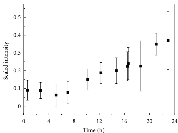
FIGURE 4: Scaled Intensity versus time for thioflavin T intensity measurements. The intensity of the emission from 10 \mu\text{M} Thioflavin T with 0.5 \text{ mg/mL} \alpha -synuclein at 520 \text{ nm} was recorded for 23 hours. The intensity was scaled by the blank measurement, and the Thioflavin T reference was subtracted from the test intensity measurement. The data shown is the average of the intensity from the two wells.
