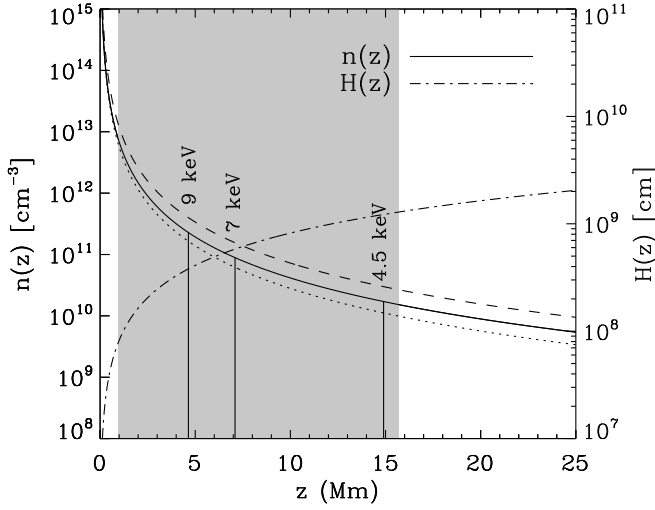
Fig. 5. Density profile required to obtain the fits shown in Figure 4. Density ( n(z) ) and local scale height ( H(z) ) versus height, z , above the footpoint are shown. The input parameters H_r , N_r and a are the best-fit parameters resulting from the fitting process outlined in Figure 4. Two alternate density models, which are derived from the alternate fits shown in Figure 4, are given here as dashed and dotted lines. The shaded region represents the range of heights within which observations of HXR sources were made, and so densities and scale heights outside of these range are not expected to be accurate. It was assumed that the density structure of the flare plasma was approximately constant over the \sim 20 s rise phase of the HXRs. Vertical solid lines indicate the location of peak emission for the denoted energies, which represent the three energy bands used in this study. The values shown correspond to the first observation, where the injection spectral index is \delta = 5 .
