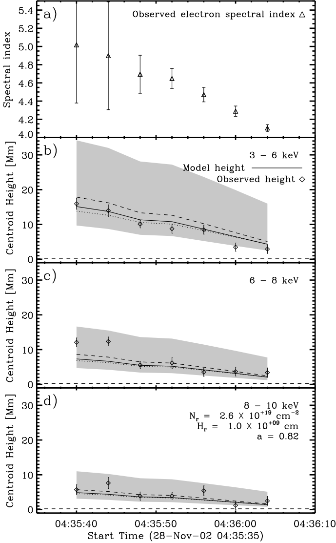
Fig. 4. (a) Electron spectral index, based on fits to RHESSI spectra. (b–d) Model and observed nonthermal source height evolutions for photon energies of 3–6 keV, 6–8 keV and 8–10 keV, respectively. Source heights derived from RHESSI observations are denoted by diamonds, with vertical solid lines indicating the 1-sigma width of the gaussian which was fit to the X-ray source. The heights corresponding to the peak in dI/dz are shown as a solid line. The shaded gray area extending above and below the solid line represents a ‘1-sigma’ width of the model intensity distribution, calculated using its full-width half-max, where FWHM = 2.35\sigma . This serves to demonstrate the size and asymmetry of the predicted X-ray source. Two alternate model height evolutions are shown as dashed and dotted lines, which use different fit parameters N_r , H_r and a . Along with the model given by the solid line, these all produce minimal \chi^2 values when fit to the data. The alternative results are presented to show the range of possible fits to the data, with corresponding density models shown in Figure 5. The dashed horizontal line represents the absolute height of the 25–50 keV footpoint, approximately 0.24 Mm. Fit parameters of the solid line are shown in section d. This model successfully accounts for a different apparent rate of descent for each emission energy, with sources observed at lower photon energy descending more rapidly.
