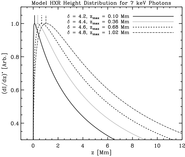
Fig. 3. Modelled HXR flux distribution with distance from the footpoint along the flare loop, produced using Equations (4) and (5), and assuming example density parameters H_r = 10^9 \text{ cm} , N_r = 2.43 \times 10^{19} \text{ cm}^{-2} and a = 0.9 . Four sample spectral index values are input, at a photon energy of 7 keV. Since z - and \delta - independent factors are neglected, the distributions are normalised such that they peak at 1, however the location of the peaks and the relative scaling between plots of different index is accurate. The height at which dI/dz distributions are at their maximum ( z_{\text{max}} ) are noted, illustrating the HXR source height's dependence on spectral index. For lower, or harder, spectral indices, the height at which dI/dz is at its maximum value is lower in the model flare loop.
