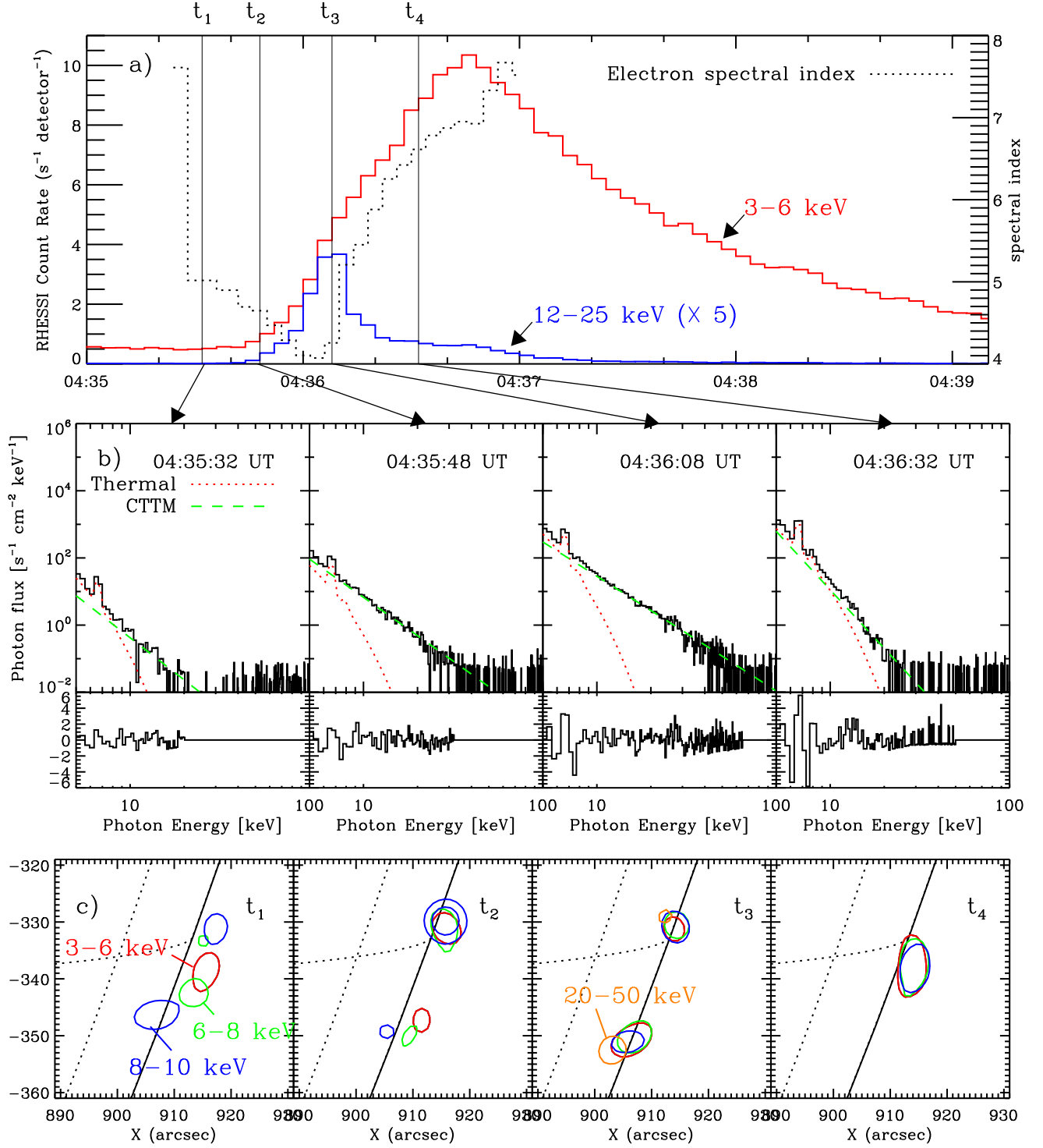
Fig. 1. (a) X-ray Lightcurve of the flare of 28 November 2002. The 12–25 keV curve is scaled by a factor of 5 for clarity. Four times are marked, corresponding to the start times of the four images and spectra shown below. Overplotted is the electron power-law index derived from the spectral fits (dotted line), demonstrating the concurrence of maximum spectral hardness (minimum spectral index) with peak in HXR emission. (b) Spatially integrated spectra for the times of their corresponding images using pre-flare background subtraction. Overlaid are thermal and nonthermal fits constructed using the OSPEX spectral analysis suite. Residuals, or the difference between observed and model-based X-ray flux, normalized to the one-sigma uncertainty in the photon flux, are plotted below each spectrum. (c) RHESSI image contours corresponding to energy bands of 3–6, 6–8, and 8–10 keV, with a contour showing 20–50 keV at t_3 , the HXR peak. Contours represent 75% of the peak emission of the image, with a second 50% contour included for the 8–10 keV image at interval t_2 , in order to show the location of the southern source. Images are generated using the CLEAN algorithm available in the RHESSI image analysis software. Each of the intervals used for these images are 8 seconds in duration, beginning at the time shown in (b).
