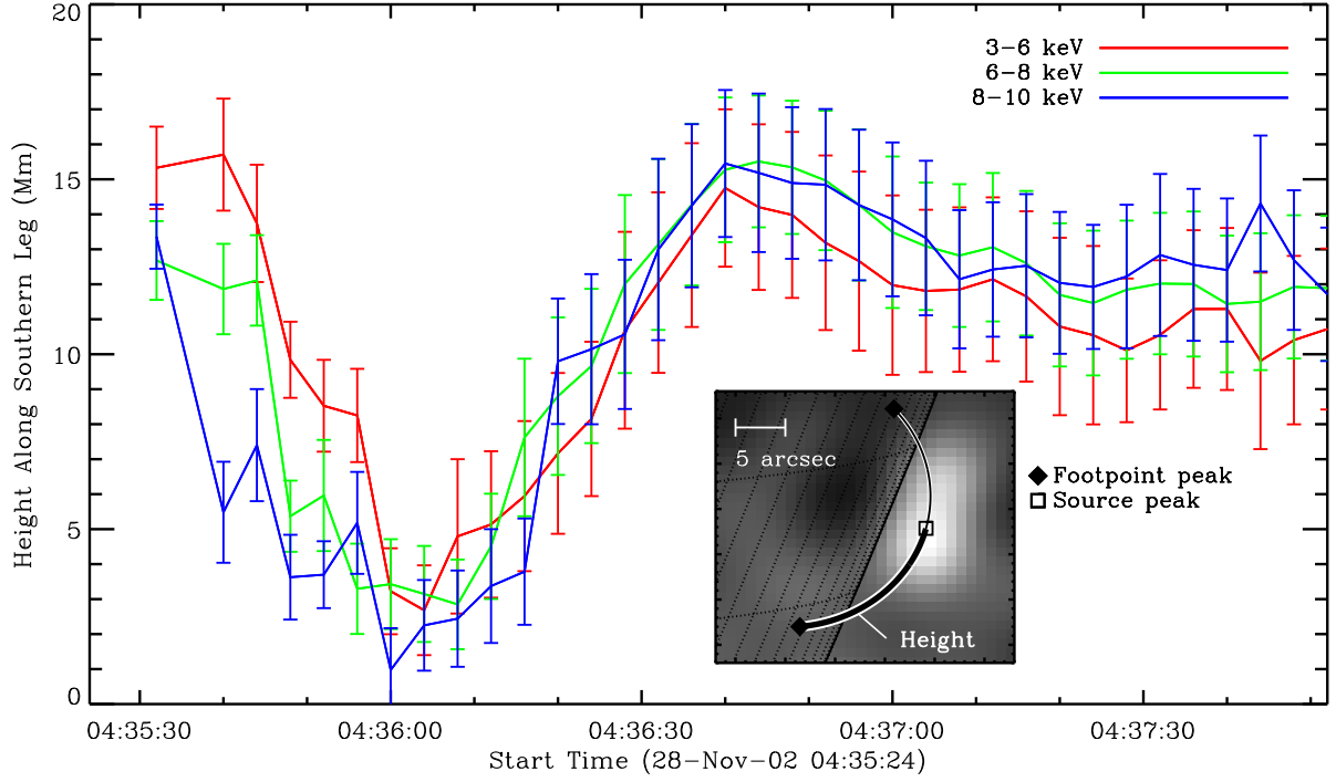
Fig. 2. Height of X-ray source peak with time for the 3–6, 6–8 and 8–10 keV energy bands. Vertical lines represent the 1-sigma width of the 2-dimensional Gaussian which was fit to the RHESSI source in order to determine peak location, thereby illustrating the size of the source, which is sensitive to the PSF of the instrument. Height is defined as distance in megametres from the source peak to the southern footpoint along the circle defined by the source peak position itself and both footpoints ( see inset ). Footpoints are defined as the peak position of 25–50 keV emission at 04:36:08–04:36:12 UT, the peak in HXRs. The temporal spacing of the data points here does not represent the integration time of the associated RHESSI images. For all images but the first, the integration time is 8 s, while the spacing between them is 4 s, resulting in an overlap of 4 s. Inset: An example image of 3–6 keV emission at 04:35:40–04:35:48 UT. The source, just prior to splitting into two, can be seen to the right of the image, at the assumed looptop. Overlaid on the image are locations of the peaks of gaussian fits to the current descending source (open square) and the 20–50 keV footpoints seen at the HXR peak (filled diamonds). The definition of height is visualised as the distance along the circle between the southern footpoint and the southern source.
