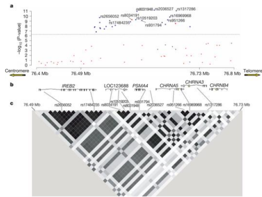
a , P -values for SNPs genotyped in the 15q25 region (76.4–76.8 Mb). The dotted line indicates the genome-wide threshold of P < 5 \times 10^{-7} . Points labelled with rs numbers have a P < 1 \times 10^{-9} . Points in red are genotyped in the 317K Illumina panel; points in blue indicate additional genotyped SNPs (Taqman). b , Positions of the six known genes. c , Pairwise r^2 estimates for 46 common SNPs from 76.49 Mb to 76.73 Mb in controls from the central Europe IARC study, with increasing shades of grey indicating higher r^2 values. The majority of pairwise D' estimates for these SNPs exceed 0.8.
