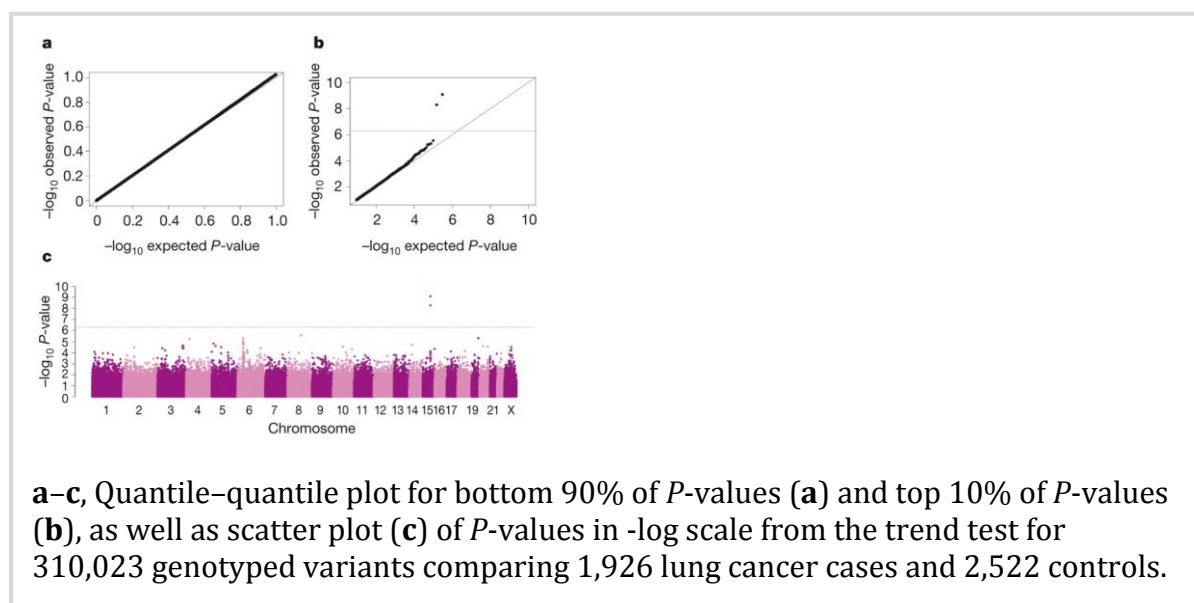
Figure 1: Genome-wide association results in the central Europe study.
