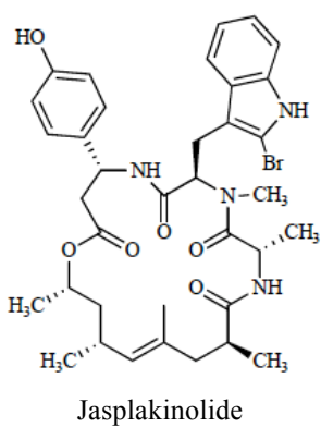
Fig. (2). Structures of some antimalarial peptides discussed in the text. Abu, L- \alpha -aminobutyrate.
