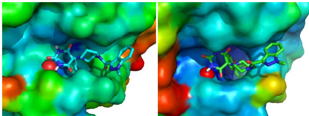
Figure 2. Pictures of 39 docked with Connolly surfaces on MMP-2 (left) and MMP-9 (right). The surfaces were generated by the programme PyMOL based on the crystal structures of MMP-2 (pdb code: 1q1b) and MMP-9 (pdb code: 2ovx). The ligand orientations were used which had the highest predicted affinity. The nitrogen atom and methyl group on the indazole of 39 were close to the amino acid Ile222/Met422 (yellow sulfur) interchange between MMP-2 and MMP-9. The active site zincs are shown as red spheres.
