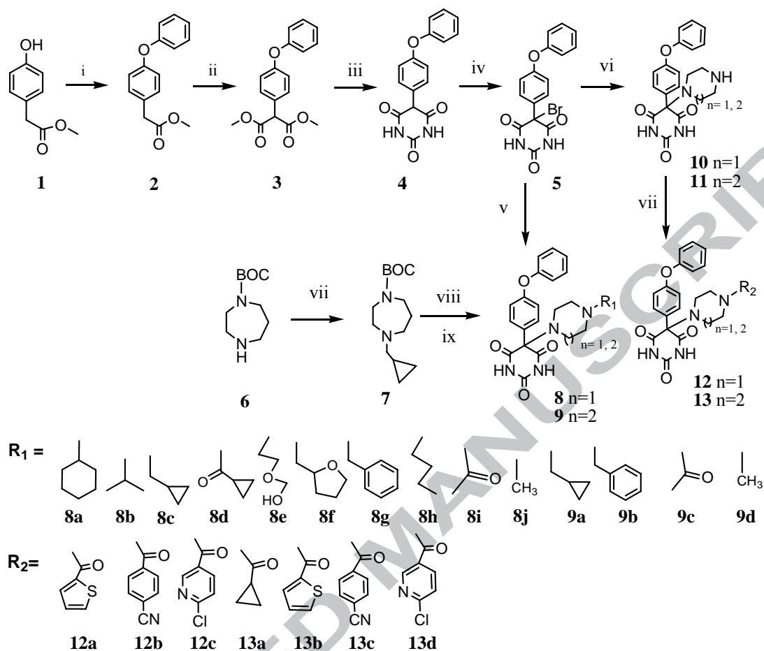
Scheme 1. Preparation of phenoxyphenyl substituted piperazine- and homopiperazine-based barbiturate derivatives. Conditions: i) C_6H_5B(OH)_2 , copper (II) acetate, pyridine, DCM, rt, 24 h, 32%; ii) (CH_3O)_2CO , NaH, dry THF, 105 °C, 5 h, 86%; iii) Na, urea, EtOH, 100 °C, 7 h, 78%; iv) Br_2 , HBr, H_2O , 0 °C, 5 h, 82%; v) substituted piperazines or homopiperazines, MeOH, rt, 24 h, 37-63%; vi) piperazine or homopiperazine, MeOH, rt, 24 h, 54-58%; vii) acid chlorides, THF, -70 °C, 5 h or carboxylic acids, DCC, DMAP, dry THF, rt, 24 h, 31-42%; viii) C_3H_5CH_2Br , MeOH, rt, 12 h, 64%; ix) CF_3COOH , DCM, 0 °C, overnight; MeOH, compounds 5, rt, 24 h, 41%.
