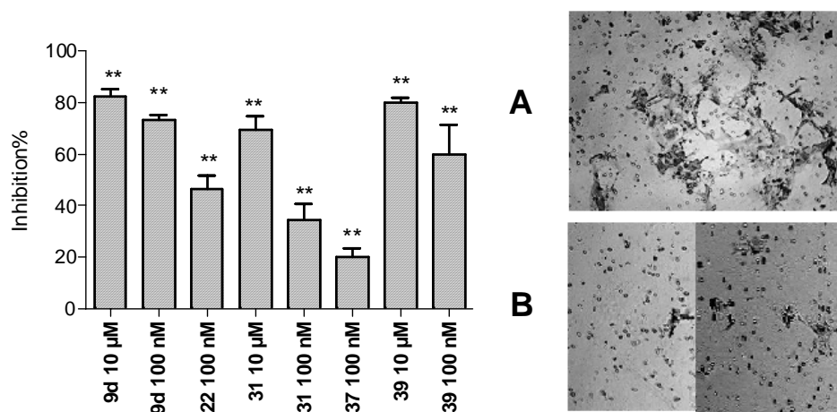
Figure 3. Results from the invasion assay with compounds 9d , 22 , 31 , 38 , 39 ( P < 0.05 ).
