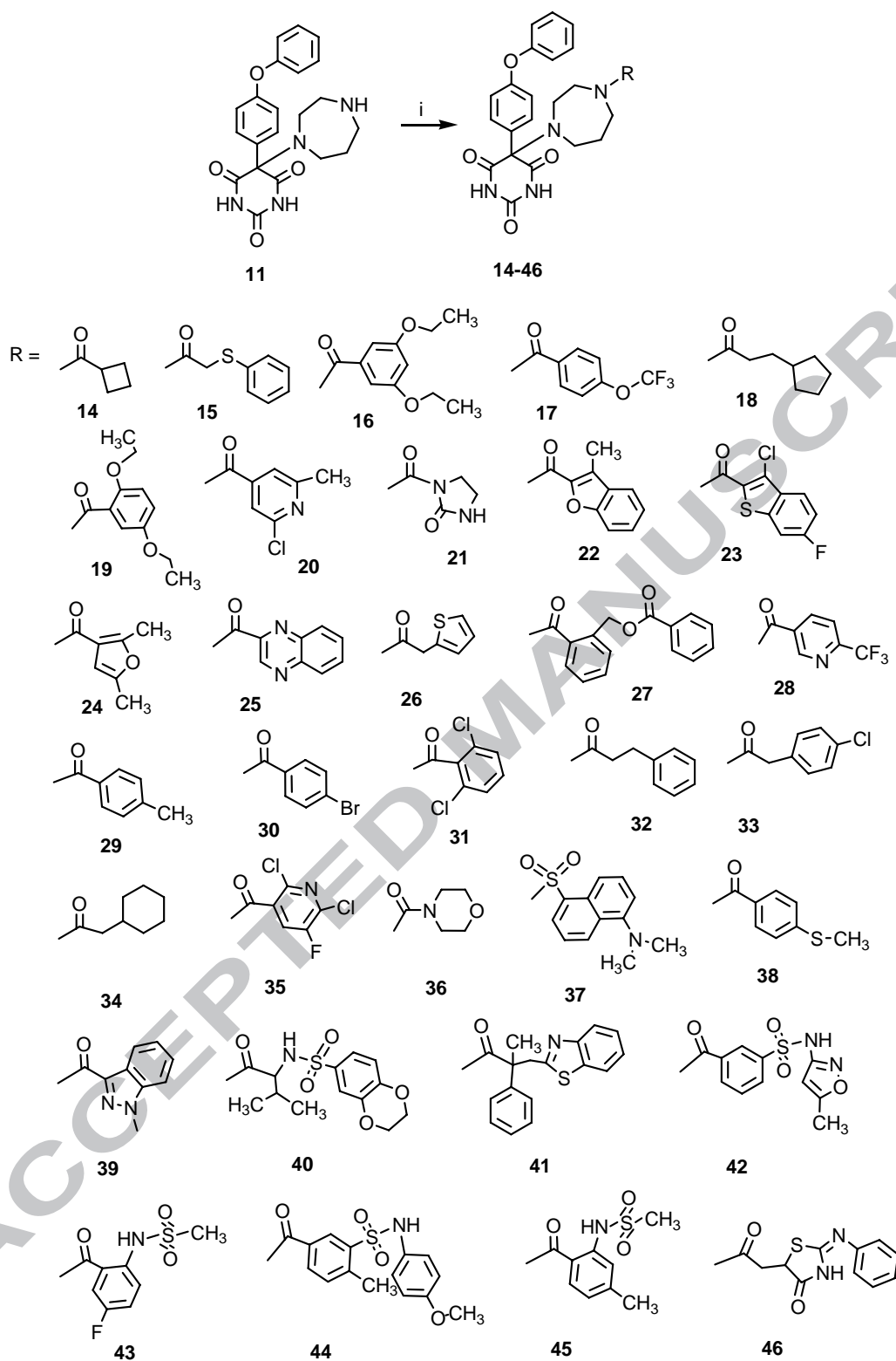
Scheme 2. Preparation of 5- N-acyl homopiperazine barbiturates. Conditions: i) acid chlorides, THF, -70^{\circ}\text{C} , 5 h. or DCC, DMAP, carboxylic acids, THF, RT, 12 h, 26-52%.
