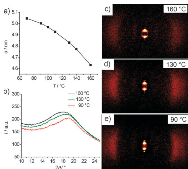
Fig. 3 XRD data of compound 1b : (a) dependence of layer distance d and (b) shape of the diffuse wide angle scattering on temperature; (c–e) diffraction pattern of a surface aligned sample (after subtraction of the scattering pattern in the Iso phase at T = 178 °C); (c) SmA at T = 160 °C; (d) SmAP R at T = 130 °C; (e) SmAP A at T = 90 °C (for original patterns, see Fig. S2, XRD patterns of compound 1a are shown in Fig. S1, ESI†).
