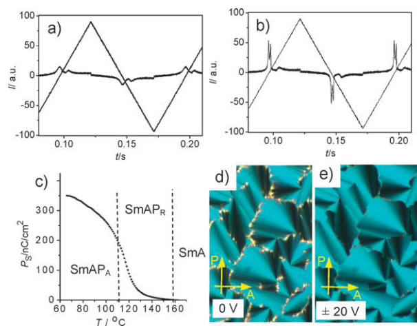
Fig. 4 Electrooptical investigation of compound 1b : (a,b) Switching current response in a 6 μm ITO cell (18 V_{pp} , 10 Hz, 5 kΩ) on applying a triangular wave field; (a) in the SmAP R phase at T = 112 °C; (b) in the SmAP A phase at T = 105 °C; (c) temperature dependence of the spontaneous polarization (9.5 μm, 20 V, 100 Hz); (d,e) textures of the SmAP R phase at 153 °C depending on applied voltage.
