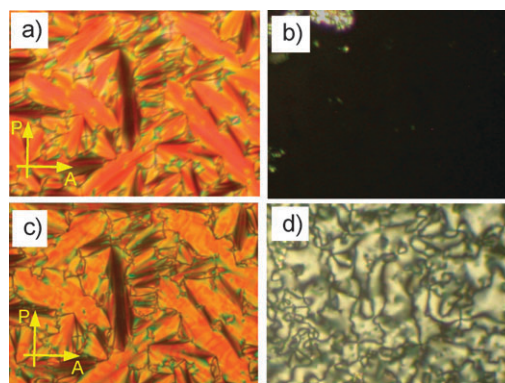
Fig. 1 Changes of the textures of compound 1a at the SmA-to-SmAP A phase transition (crossed polarizers); (a,b) SmA phase at T = 130 °C; (c,d) SmAP A phase at T = 100 °C; (a,c) fan-like texture; (b,d) homeotropically aligned sample.
