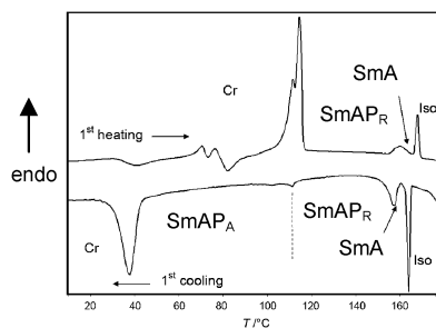
Fig. 2 DSC heating and cooling curves (10 K min -1 ) of compound 1b .
