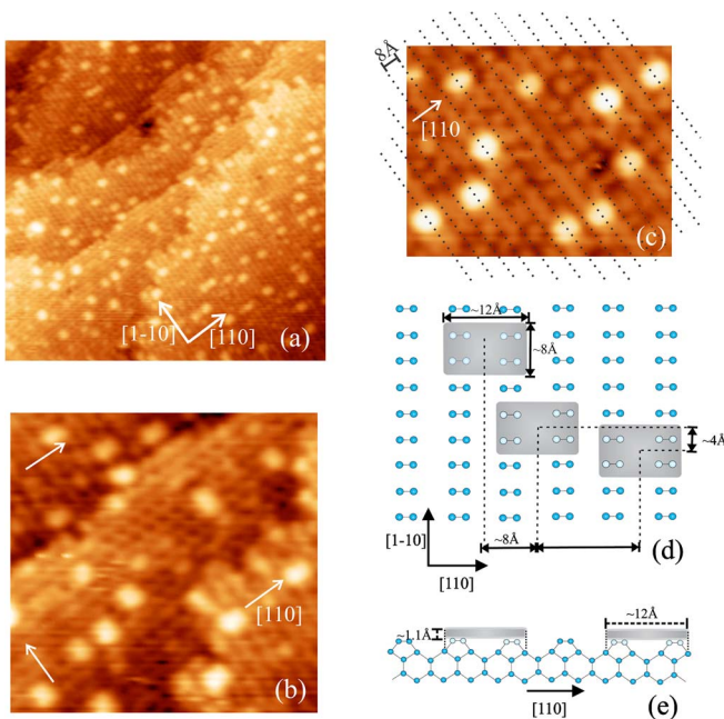
FIG. 2. (Color online) (a) 370 \times 370 \text{ \AA}^2 empty state STM image of Ge(001) surface following deposition of \sim 0.08 \text{ ML Fe} . (b) 135 \times 135 \text{ \AA}^2 STM zoom in, showing the dots, elongated across the dimer rows, rotate from one terrace to the next. (c) 110 \times 90 \text{ \AA}^2 STM image. The dashed lines along [1\bar{1}0] are separated by 8 \text{ \AA} . These lines always pass through the center of the dots, illustrating the definite registry of the dots with the substrate. The loss of long range (2 \times 1) symmetry, characteristic of clean Ge(001), is also evident from this image. (d) Model of registry of the Fe dots on the (2 \times 1) Ge(001) surface. As a result of the observed spacing, it can be concluded that all dots nucleate at equivalent positions, as shown here. (e) Side view of dots with respect to the surface.
