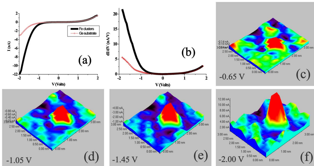
FIG. 3. (Color online) (a) I(V) tunneling spectra over Fe dots (thick solid) and surrounding Ge (001) substrate (thin circles). Marked current rectification due to the dots is evident. (b) Derivative of I(V) spectra. Dots have band gap \sim 0.65 \text{ V} , and surrounding substrate \sim 0.75 \text{ V} . [(c)–(f)] I(V) map obtained over a single Fe dot. Current rectification is well confined to area over the dot. No change in tunneling behavior of surrounding substrate observed.
