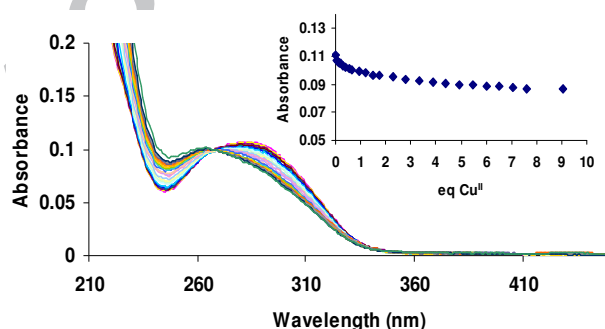
Figure 2. The overall changes in the absorption spectra (uncorrected) of 1.Tb.Na (10 \mu M) upon titration with Cu(HClO 4 ) 2 in deionised H 2 O. Inset: Changes observed at 285 nm as a function of equivalents of Cu(II) added
