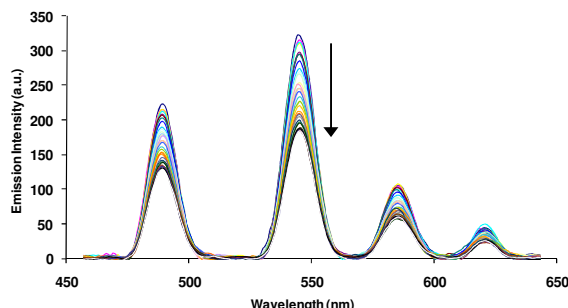
Figure 5. Changes in the Tb(III) luminescence spectra of 1.Tb.Na (10 \mu\text{M} ) upon titration with \text{Hg}(\text{HClO}_4)_2 (being quenched) in deionised \text{H}_2\text{O} (0 \rightarrow 100 \mu\text{M} ).
