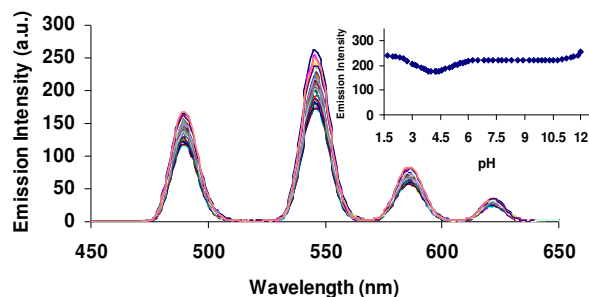
Figure 1. The overall changes in the Tb(III) luminescence of 1.Tb.Na (10 \mu\text{M} ) upon excitation of the phenyl antenna ( \lambda_{\text{ex}} = 285 nm) as a function of pH ( I = 0.1 M \text{NEt}_4\text{HClO}_4 (TEAP)). Inset : The changes at 545 nm vs. pH.
