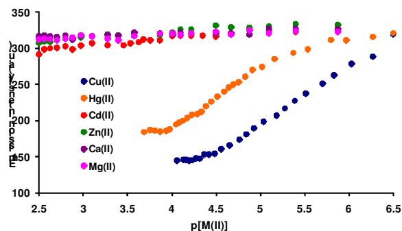
Figure 4. Plot of the changes in the Tb(III) luminescence of 1.Tb.Na (10 \mu\text{M} ) at 545 nm upon titration with \text{M}(\text{HClO}_4)_2 or \text{MCl}_2 (expressed as \text{pM} = -\log[\text{M}] ) in deionised \text{H}_2\text{O} .
